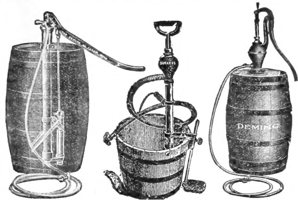
DEMING'S "CENTURY" BARREL SPRAY PUMP PERFECT SUCCESS BUCKET PUMP DEMING'S "SIMPLEX" BARREL SPRAY PUMP
