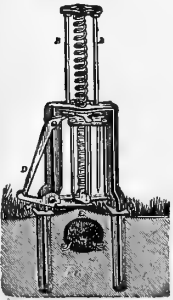
Olmstead's Mole Trap
