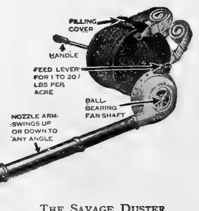
THE SAVAGE DUSTER
