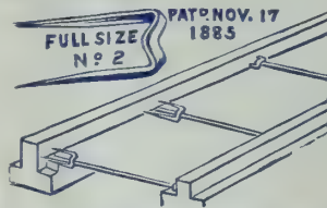
THE VAN REYPER GLAZING POINT.
