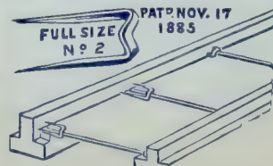
THE VAN KEYSER GLAZING POINT.
