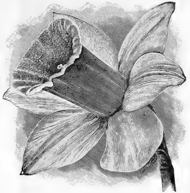
NARCISSUS HORSFIELDI
