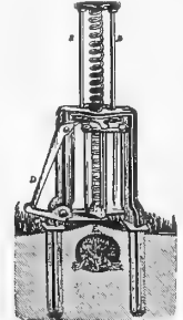
Schroeter Mole Trap
