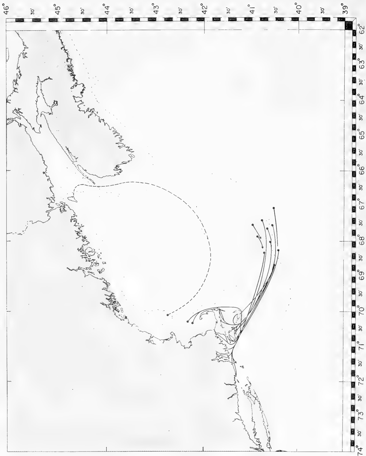
FIGURE 17. --Surface circulation deduced from recoveries of drift bottles launched on Albatross III Cruise 110 and Metacomet Cruise 58-2, May 6-11, 1958.
