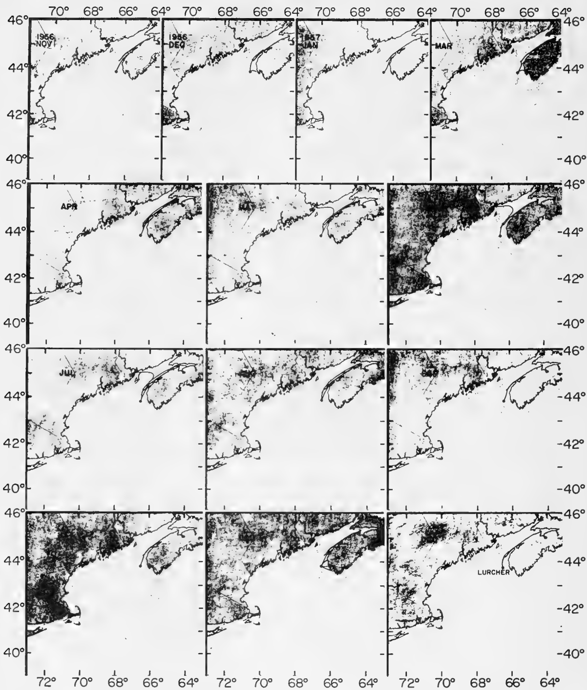
FIGURE 23.--Surface circulation deduced from recoveries of drift bottles launched from Lurcher Lightship each day during the period October 9, 1956-December 31, 1957.
