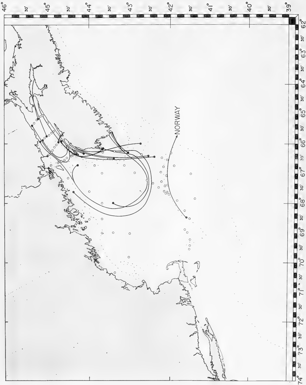
FIGURE 11. --Surface circulation deduced from recoveries of drift bottles launched on Harengus Cruise 18 and Albatross III Cruise 104, October 7-25, 1957.
