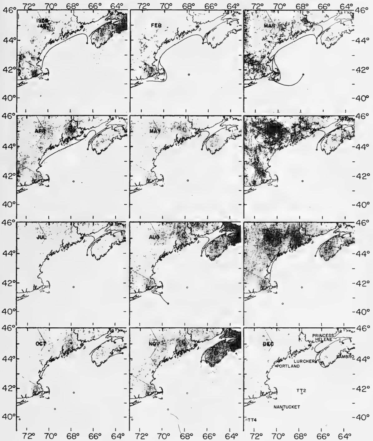
FIGURE 24.--Surface circulation deduced from recoveries of drift bottles launched from several positions each day during 1958.
