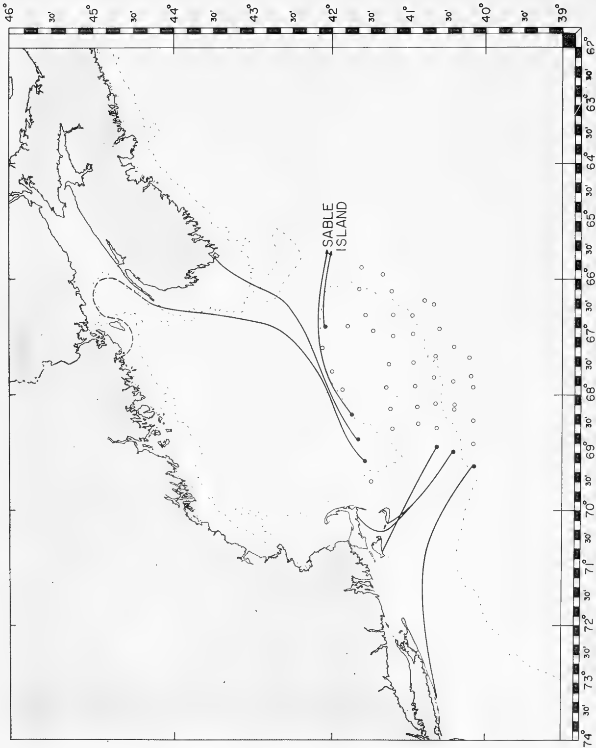
FIGURE 9. --Surface circulation deduced from recoveries of drift bottles launched on Albatross III Cruise 95, June 5-9, 1957.
