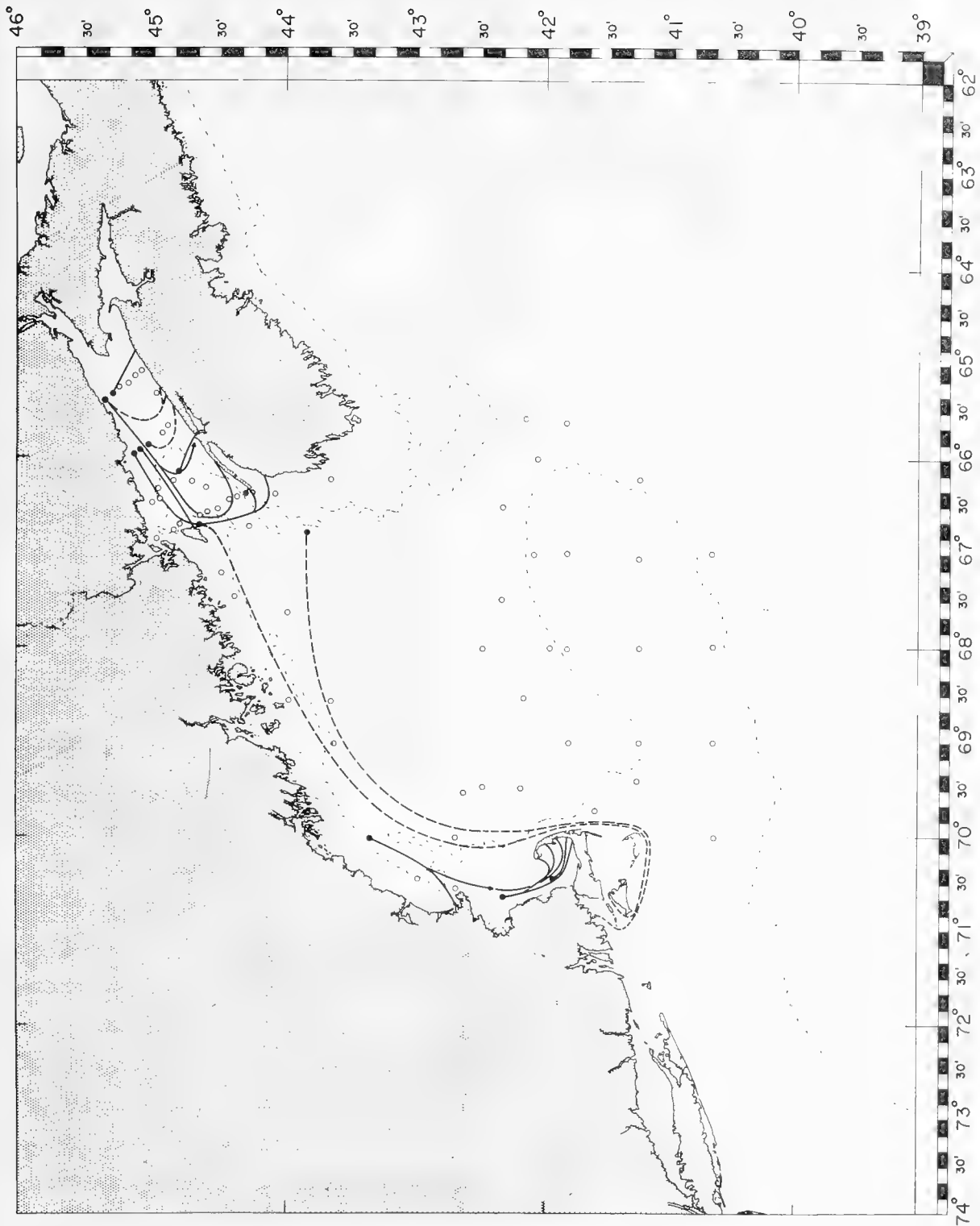
FIGURE 14. --Surface circulation deduced from recoveries of drift bottles launched on Albatross III Cruise 107 and Delaware Cruise 57-9 (111). January 18-29, 1958.
