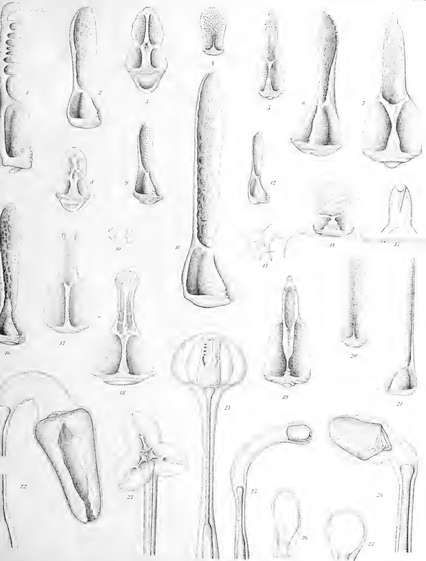
Parechinus, Lozechinus, Paracentrotus, Stomopneustes.
