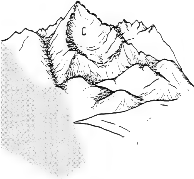
Figure B-6 —Diagram including a cirque (C) (adapted from Land System Inventory Handbook, USDA Forest Service, R10. 1982).
