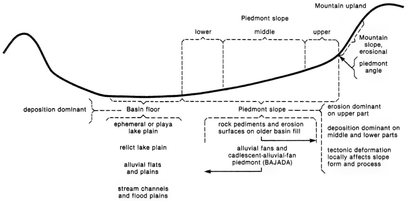
Figure B-3—Bolson and included landforms (adapted from Gile, et al. 1981).
