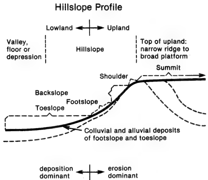
Figure B-2—Hillslope components in profile (adapted from Gile and others. 1981).
