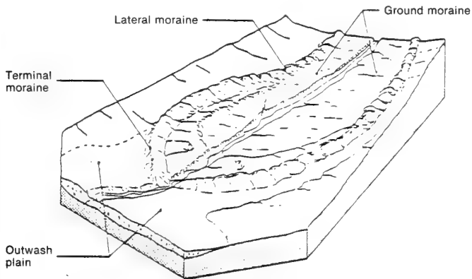
Figure B-7 —Schematic block diagram showing some glacial features (from: Landform Units; common to the Bitterroot, Clearwater, Lolo, and Nez Perce National Forests as used in Land Type Mapping; U.S. Forest Service; Region 1).
