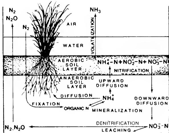
Figure 63. A schematic outline of the redox zones in a submerged soil showing some of the N transformations (Copyright. Reprinted from "Nitrogen in Agricultural Soils," 1982, with permission of the American Society of Agronomy). The aerobids layer has been drawn thick for clarity. In reality, it is seldom over 1-2 mm in flooded marshes.
