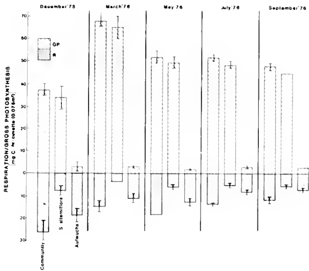
Figure 61. Carbon dioxide flux measurements in a deltaic salt marsh community (unpublished data; see Gosselink et al. 1977).
