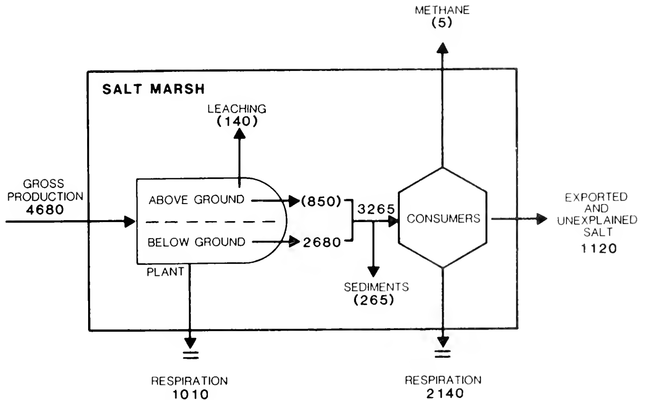
Figure 62. Carbon budget of a Mississippi River deltaic salt marsh (see Table 29 for sources). Rates ( \text{g C}/\text{m}^2/\text{yr} ) are from \text{CO}_2 flux measurements, except numbers in parentheses, which are from other sources.
