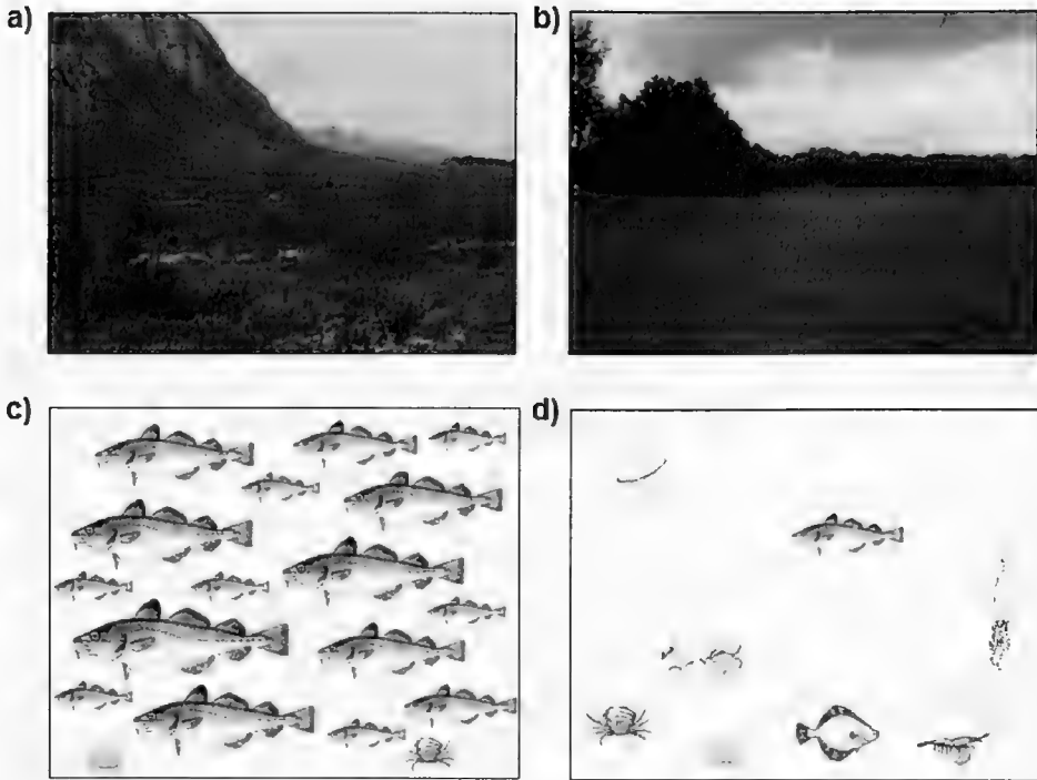
Figure 1 Illustration of the importance of variability and of amount for the provisioning of different benefits from nature. a) High variability, low biomass fynbos ecosystem. b) Low variability, high biomass improved pasture. Despite its lower biomass, the fynbos ecosystem has a higher value for the provisioning of benefits that depend on diversity, such as compounds for the pharmaceutical industry. c) High biomass, low variability cod-dominated marine system. d) Low biomass, high variability marine system after overexploitation of cod. Despite its lower variability, the cod-dominated system has a higher value for the provisioning of food, a benefit that is highly sensitive to amount (biomass).
