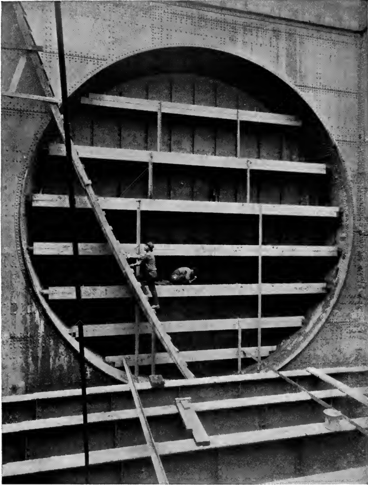
LAND SHAFT CAISSON AT SPRING STREET, NEW YORK CITY Showing steel bulkhead in west side wall through which shield advanced after erection
