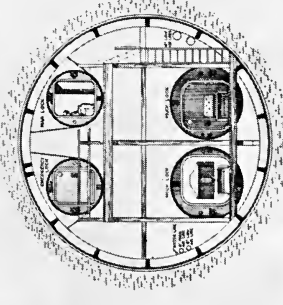
EXTERIOR VIEW OF CONCRETE BULKHEAD SHOWING AIR LOCKS
