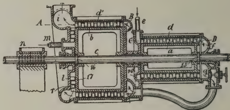
718,661. Steam Turbine.
