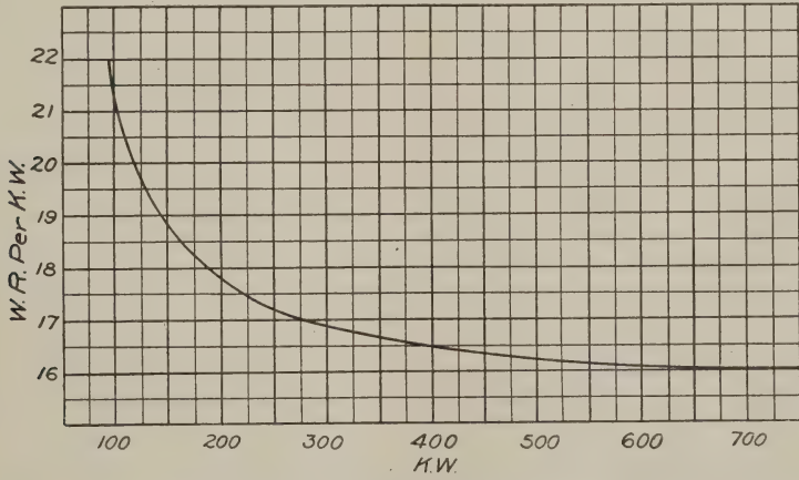
CURVE 2. Curve Showing Water Consumption, in pounds per K.W., of 600 K.W. Curtis Steam Turbine, at Different Outputs when operating at 1,500 R.P.M.; Vacuum 28.5" and a Steam Pressure of 200 lbs., which is Superheated to 150° Fahr.
