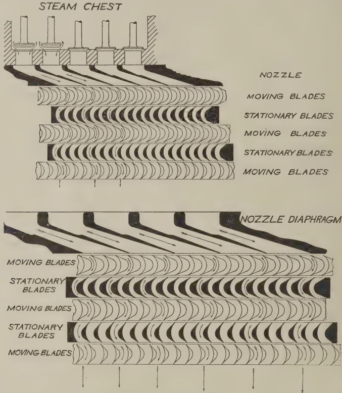
Diagram of Nozzles and Buckets.
