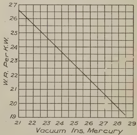
CURVE 5. Curve Showing Water Consumption, in pounds per K. W. of 600 K.W. Curtis Steam Turbine, for Different Vacua as Measured in Inches of Mercury. Turbine Operating at 1,500 R.P.M., under a pressure of 140 lbs. of Steam and Delivering 600 K.W.
