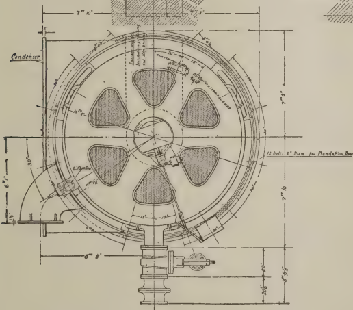
Plan and Elevation of 5,000 K.W. Curtis Turbine With Generator.
