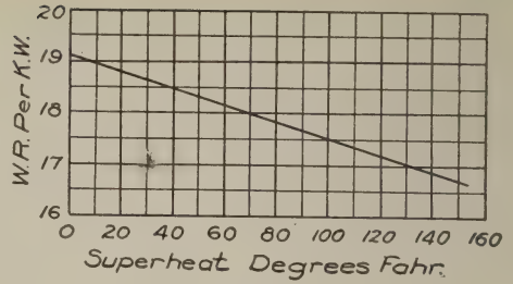
CURVE 4. Curve Showing Water Consumption, in pounds per K. W., of 600 K.W. Curtis Steam Turbine, at Different Degrees of Superheating, when operating at 1,500 R.P.M.; Vacuum 28.5"; Pressure 140 lbs., and Delivery 600 K.W.
