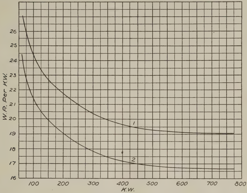
CURVE 1. Comparative Curve Showing Water Consumption, in pounds per K.W., of 600 K.W. Curtis Steam Turbine, when operating at 1,500 R.P.M., Under 140 lbs. Pressure and a Vacuum of 28.5". 1. Without Superheat. 2. At 150° Fahr. Superheat.
