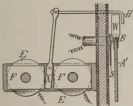
E -ELECTRO-MAGNET. H -HOOK. F -POLE-PIECES. X -ARMATURE.
