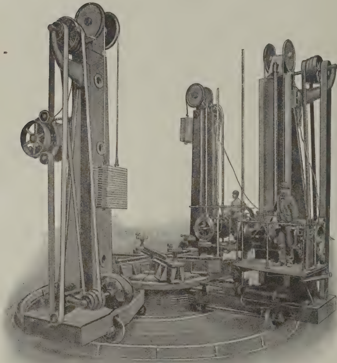
Alternating Current Motor Driving Group of Boiler Shell Drills.
