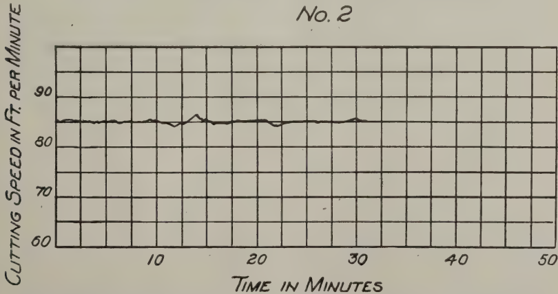
Cutting Speeds and Time Required to Face a 72 inch Cast Iron Disc with Lathe Driven by Motor with Field Control.
