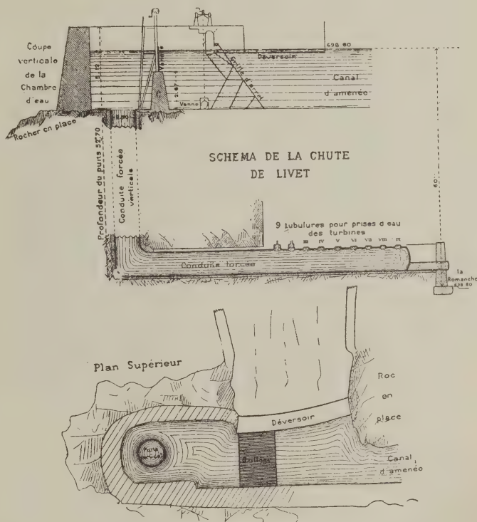
Canal and Tunnel at Livet.
