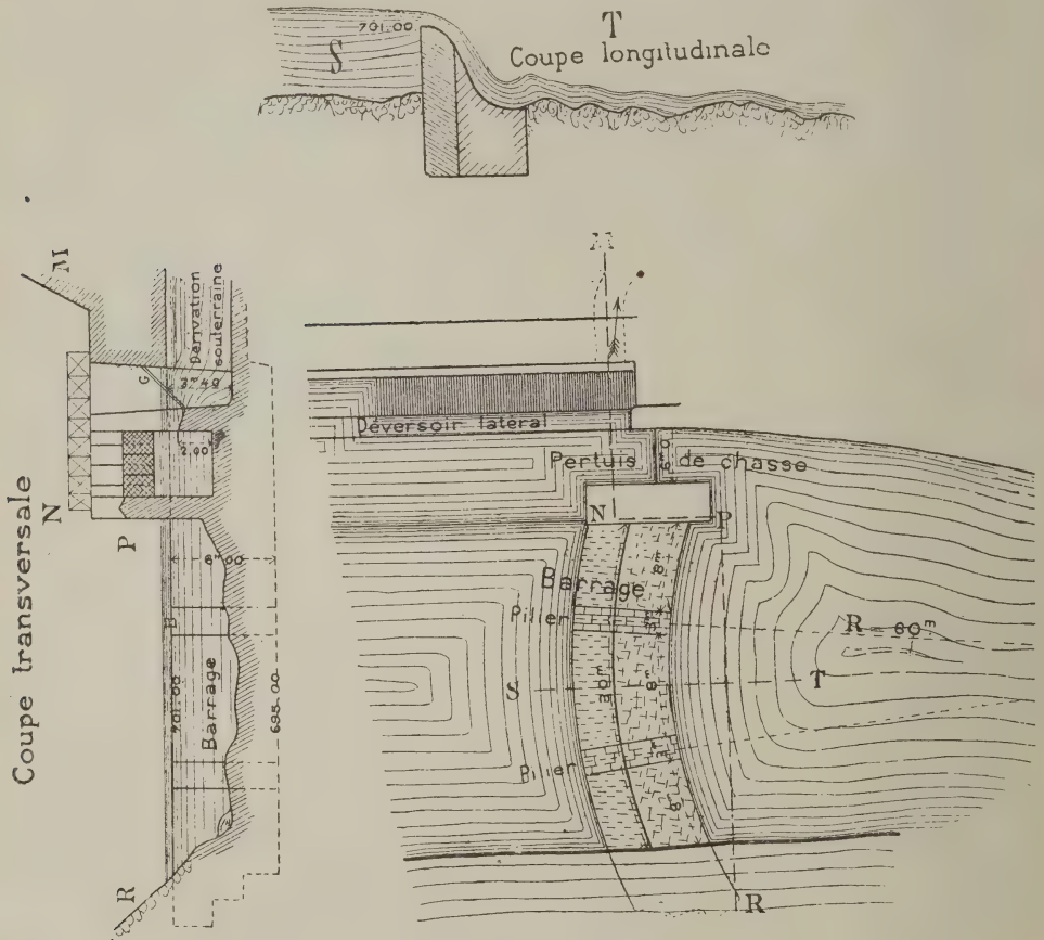
Plan of the Dam at Livet.
