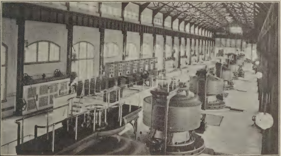
Five-thousand Horse Power Generators in Niagara Falls Power Company's Power House.
