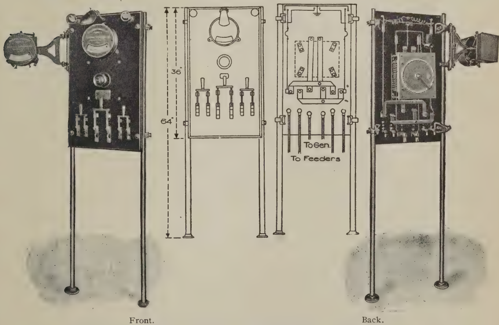
Small Plant Switchboards. Showing Front and Back Views and Wiring Connections.
