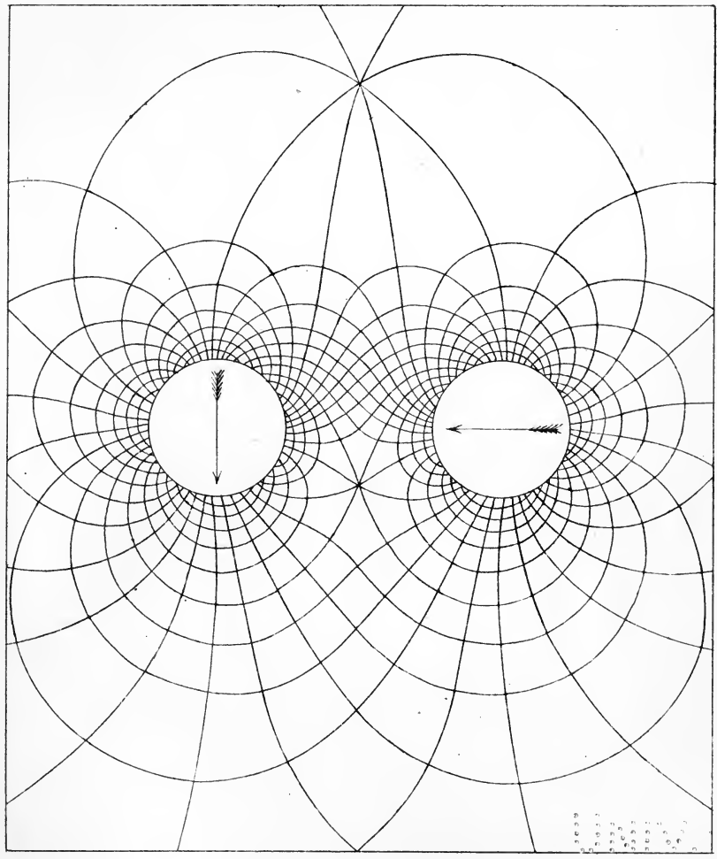
Two Cylinders magnetized transversely.
