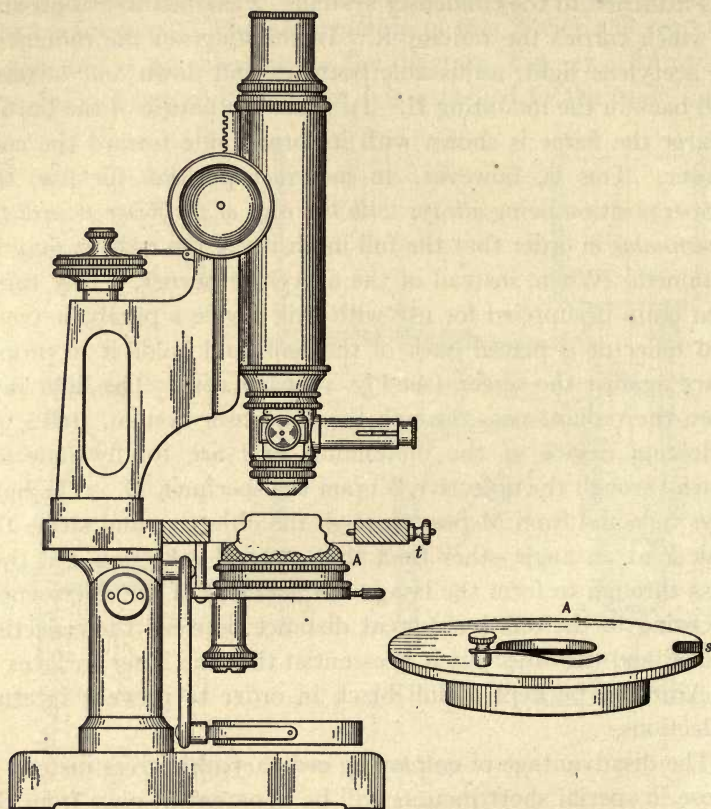
FIG. 38. Chemical Microscope with Stage removed and Auxiliary Stage inserted in the Substage Ring.
