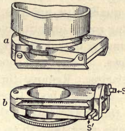
FIG. 102. Zeiss Centering Objective Changer.
