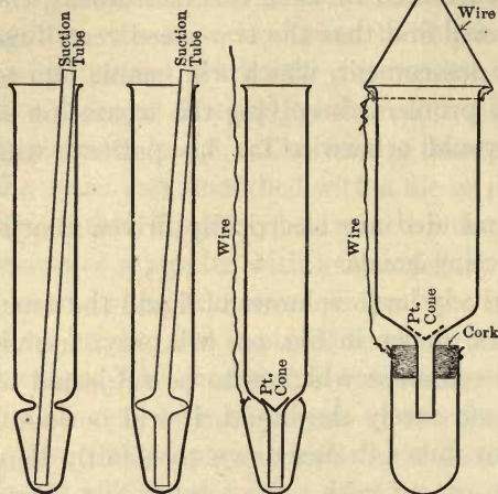
FIG. 147. Richards Tubes for Centrifugal Separations.
