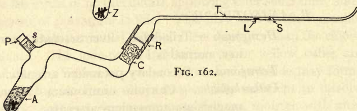
Apparatus for the Detection of Arsenic.
