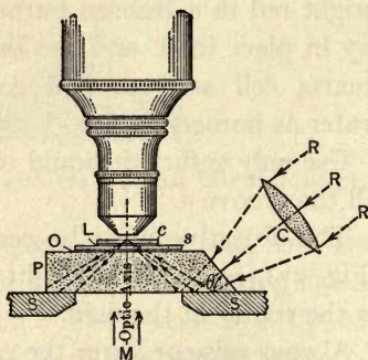
FIG. 59. The Ultramicroscope of Cotton & Mouton.
