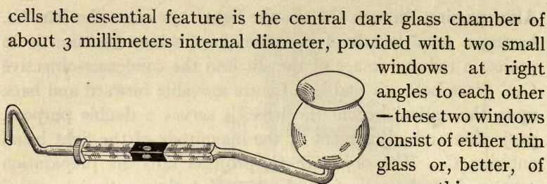
FIG. 53. Biltz-Thomae Cell.
