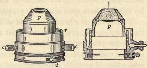
FIG. 20. Paraboloid Dark-field Illuminator.
