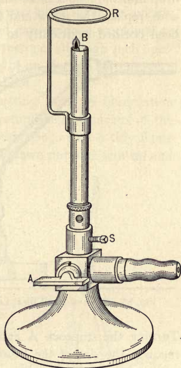
FIG. 87. Burner for Microchemical Analysis. ( \times \frac{1}{2} .)
