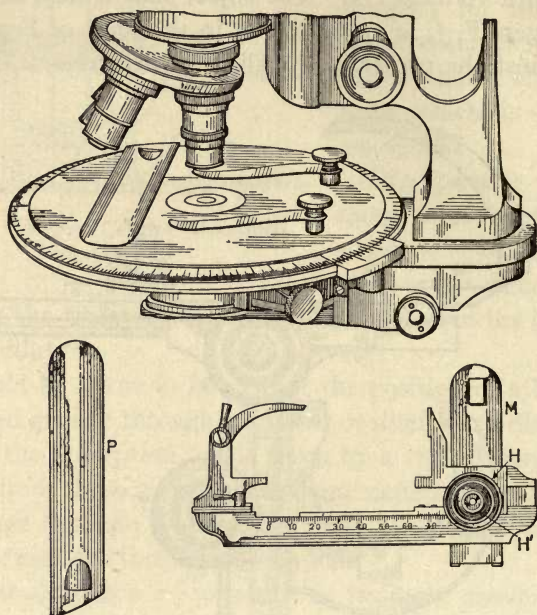
FIG. 71. Removable Mechanical Stage. Spencer Lens Co.
