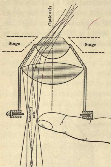
FIG. 5. Diagram of Abbe Condenser; Oblique Light.
