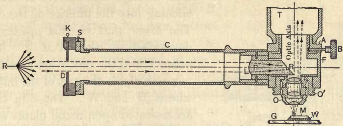
FIG. 34. Nachet Vertical Illuminator.
