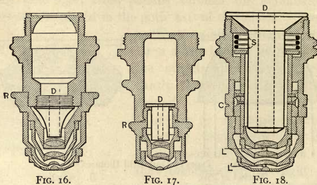
FIG. 16. FIG. 17. FIG. 18. Methods of Reducing Numerical Aperture of Objectives for Dark-field Studies. (D, D, D, Removable Diaphragms.)
