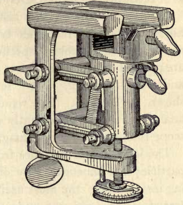
FIG. 106. Small "Table" Microtome. Spencer Lens Co.
