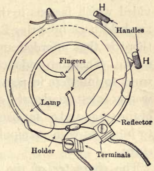
FIG. 9. Silverman Illuminator. Lamp and Holder.
