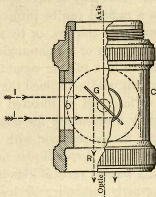
FIG. 33. Disk Vertical Illuminator.
