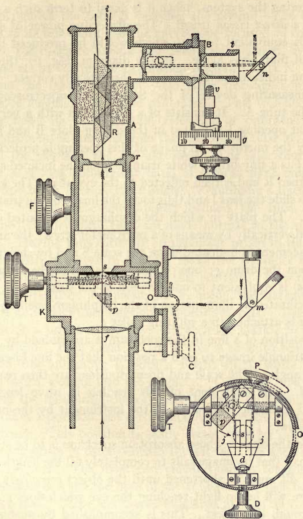
FIG. 67. Microspectroscope.
