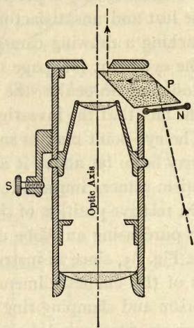
FIG. 65. Drawing Eyepiece. (E. Leitz.)
