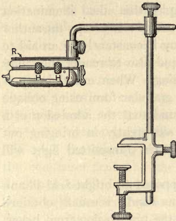
FIG. 11. Clamp for holding Silverman Illuminator below objectives when used with Greenough type Binocular Microscopes.
