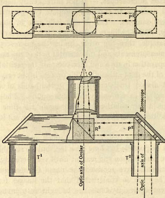
FIG. 27. The Bausch and Lomb Comparison Eyepiece.
