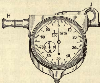
FIG. 105. B. C. Ames Co. Dial Gauge.
