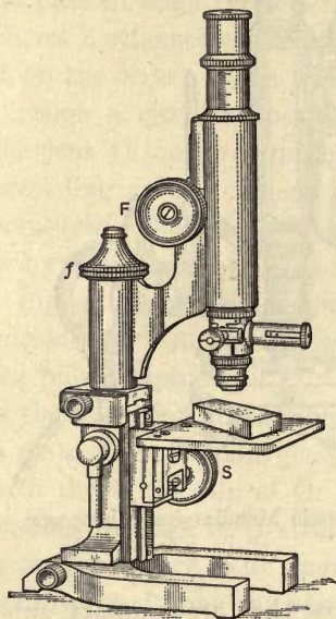
FIG. 48. Leitz Metallurgical Microscope.
