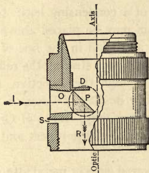
FIG. 32. Prism Vertical Illuminator.
