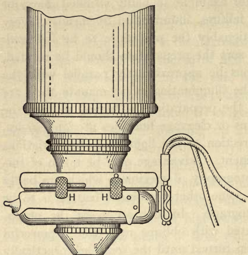
FIG. 10. The Silverman Illuminator attached to the Objective of the Microscope.
