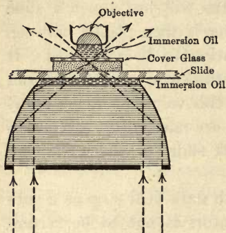
FIG. 13. Dark-field Illumination.
