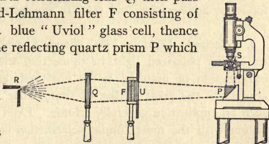
FIG. 21. Reichert Fluorescence Microscope.
