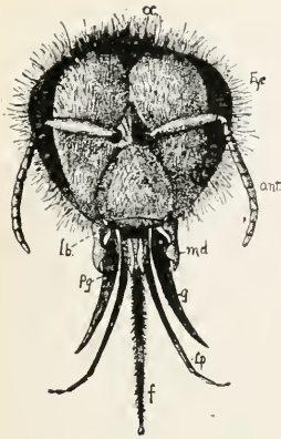
FIG. 64. Head and mouth-parts of worker bee. Eye , compound eye; ant , antennæ; lb , labium; md , mandible; g , maxilla; lp , labial palpi; pg , paraglossa; f , tongue or glossa.
