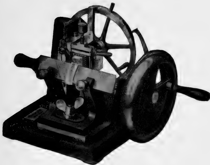
FIG. 5.—Rotary Microtome. (Leitz.)
