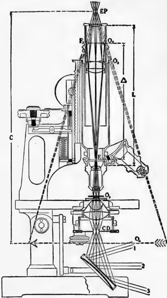
FIG. 18.—Diagram Showing Path of Light Rays.
