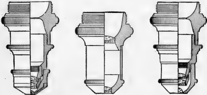
FIG. 19.—Sectional Views of Objectives. (Bausch & Lomb.)
