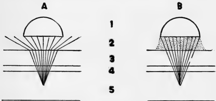
FIG. 20.—Immersion Objectives.
