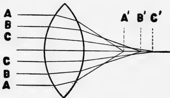
FIG. 13.—Spherical Aberration.
