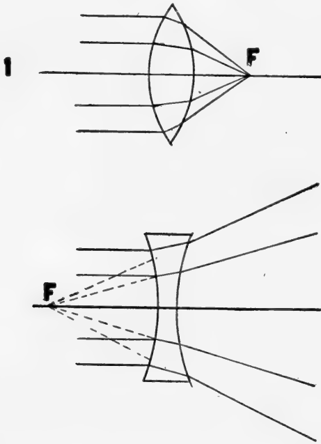
FIG. 10.—Refraction of Light Rays by Lenses.
