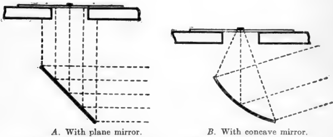
FIG. 23.—Illumination of Object by Mirror, without Condenser.
