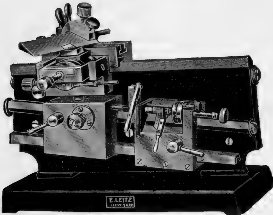
FIG. 4.—Sliding Microtome. (Leitz.)
