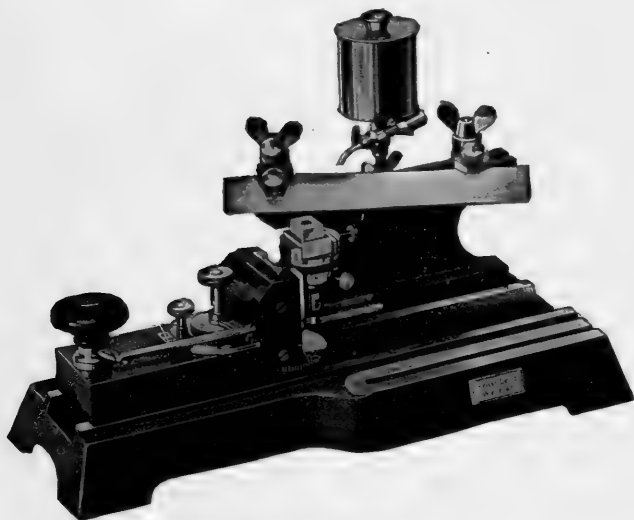
FIG. 6.—Sliding Microtome. (Leitz.)
