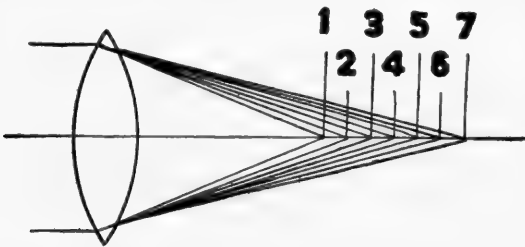
FIG. 14.—Chromatic Aberration.
