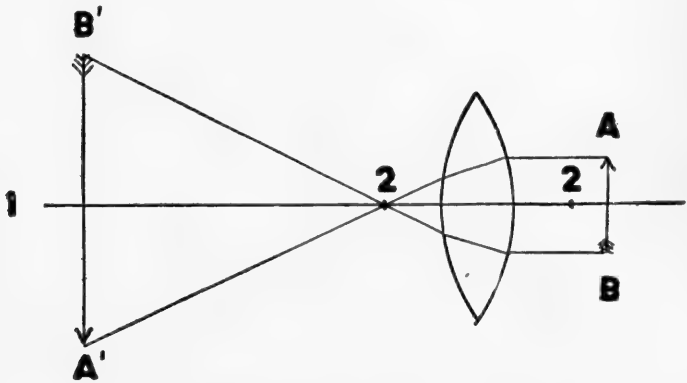
FIG. 11.—Formation of Real Image by Convex Lens.
