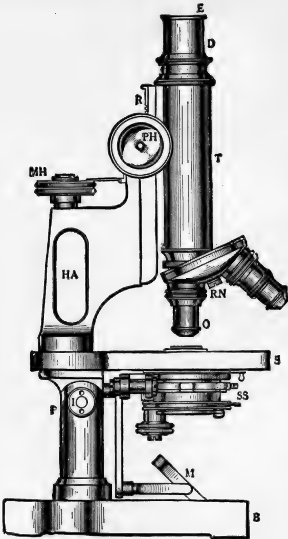
FIG. 22.—Parts of the Compound Microscope.
