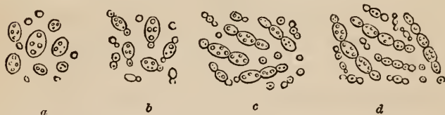
Yeast-plant ( Torula cerevisiæ ) as developed during fermentation.
