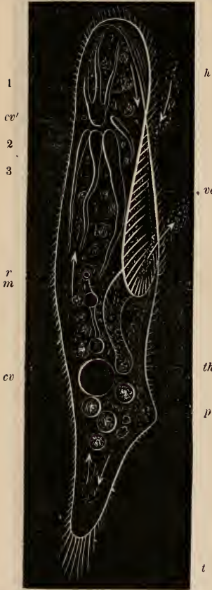
Paramecium caudatum , Ehrenberg —Magnified.
