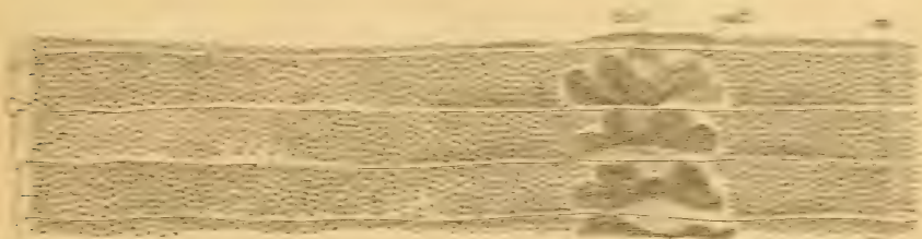
FIG. 26.—Transverse view of lateral half of a few segments of same, \times 10 . A median line; an oral; an sucker; the numerous dot-like bodies on either side of the center represent the polar granules. \times 10 . After Jima & Kamada, 1894, p. 5.
