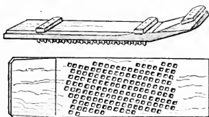
FIG. 10.—Syrian threshing-sledge. After Benzinger.
