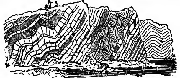
FIG. 5.—Curved and Contorted Rocks, near Old Head of Kinsale. (Du Noyer.)
