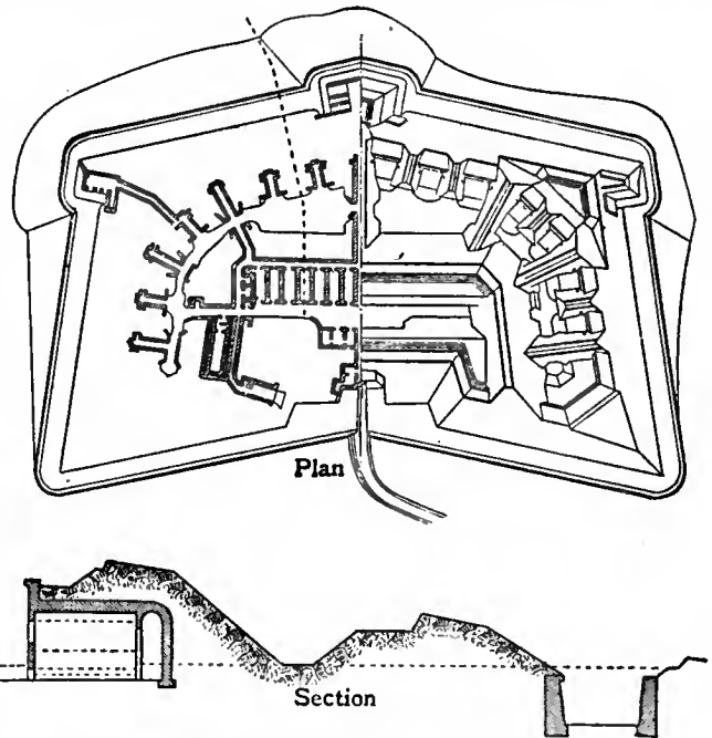
FIG. 43.—French Fort about 1880.
