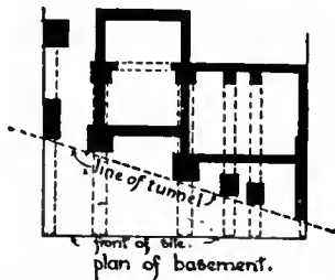
FIG. 13.—Cantilever Foundation over Railway Tunnel.
