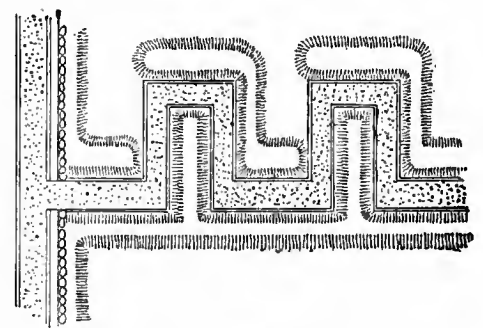
FIG. 69.—Direct advance by Double Sap.
