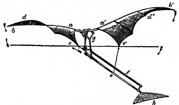
FIG. 40.—Pénaud's Artificial Flying Bird.
