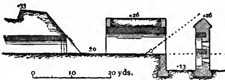
FIG. 35.—Mortar-casemate and Detached Wall.
