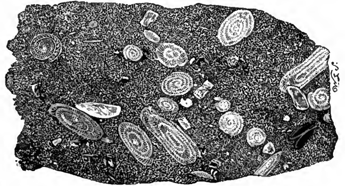
FIG. 20.—Section of Fusulina Limestone.
