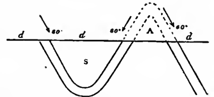
FIG. 17.—Section along the downcast side of same fault.
