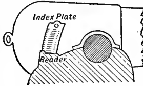
FIG. 18.—Sketch of Index Plate and Reader.
