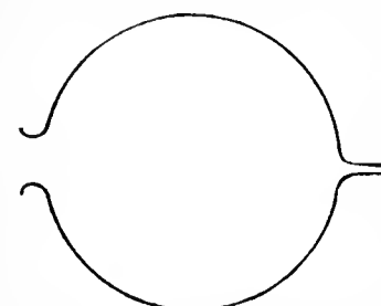
FIG. 24.—Helmholtz Resonator.
