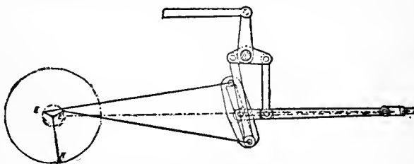
FIG. 31.—Allan's Link-Motion.
