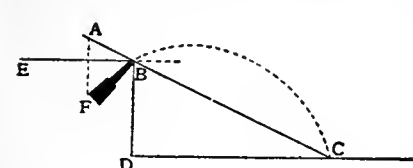
FIG. 19.—Theory of the Automatic Sight.
