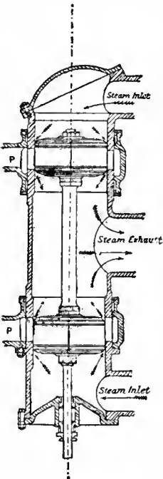
FIG. 40.—Piston Slide-Valve.
