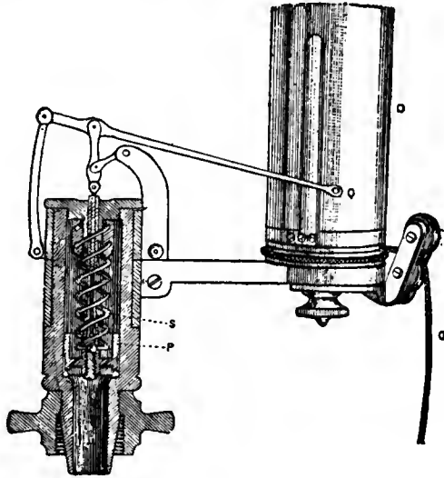
FIG. 15.—Crosby Indicator.
