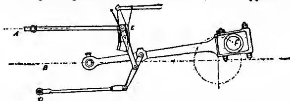
FIG. 36.—Joy's Gear as applied to a Locomotive.
