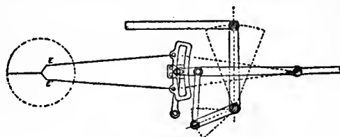
FIG. 30.—Gooch's Link-Motion.
