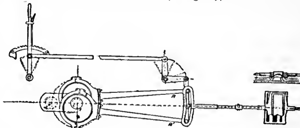
FIG. 29.—Stephenson's Link-Motion.
