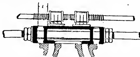
FIG. 37.—Expansion-Valve on back of Main Slide-Valve.
