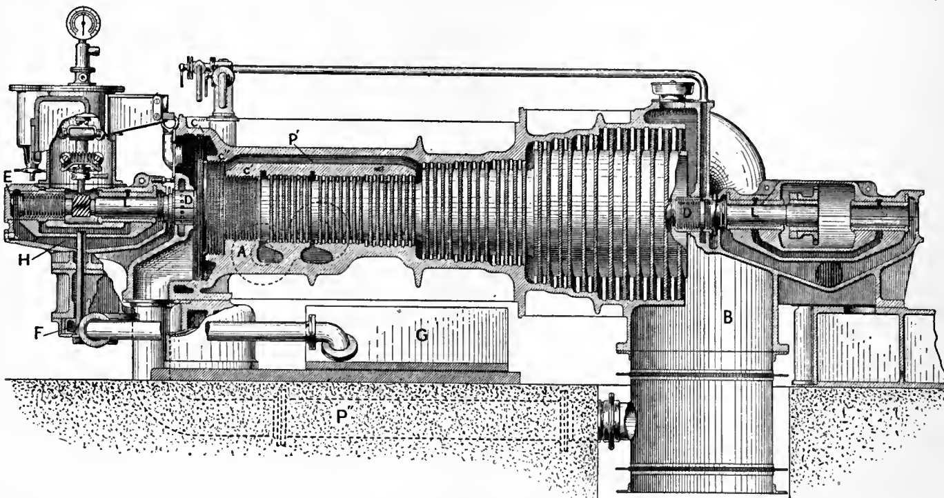
FIG. 60.—Parsons Turbine.
