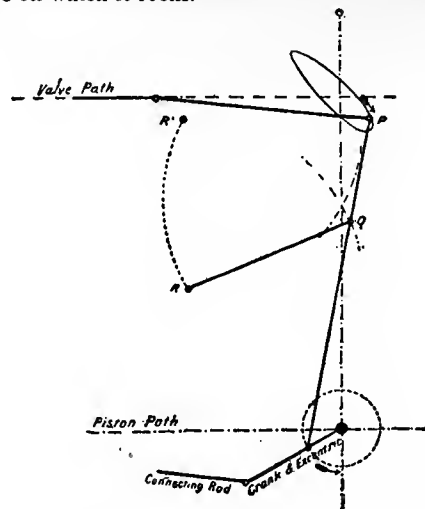
FIG. 34.—Bremme's or Marshall's Valve-Gear.
