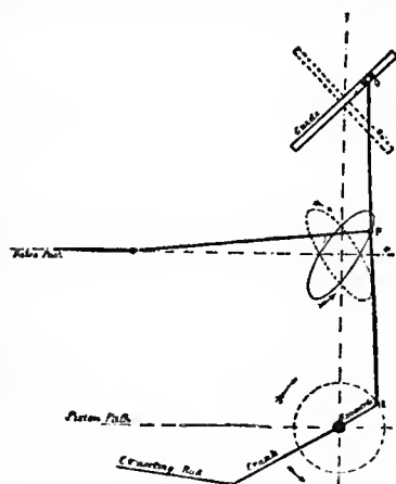
FIG. 33.—Hackworth's Valve-Gear.
