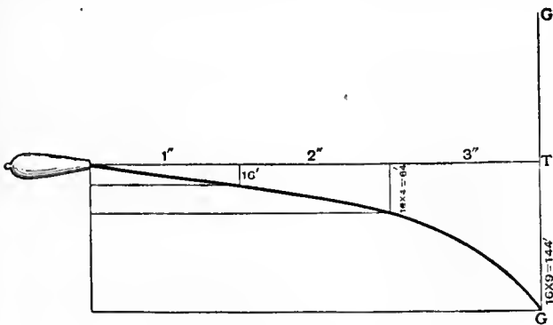
FIG. 1.—Elevation.
