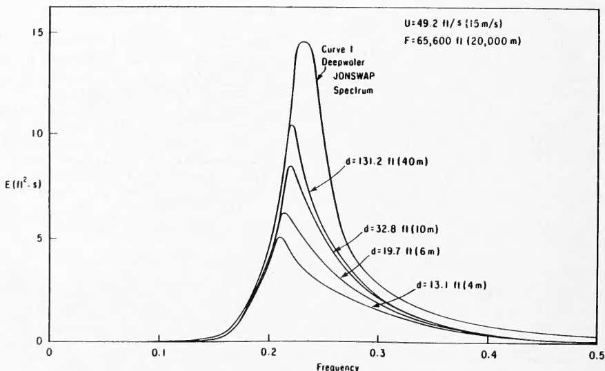
Figure 1. Transformation of JONSWAP spectrum in shallow water.
