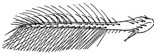
Fig. 4.—Left forewing.
