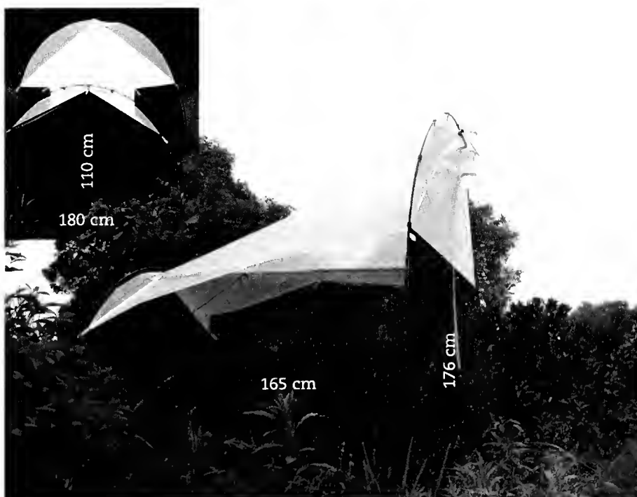
12. Bugdorm design of Malaise trap with rounded roof and no rods. Photo: C. van Achterberg
