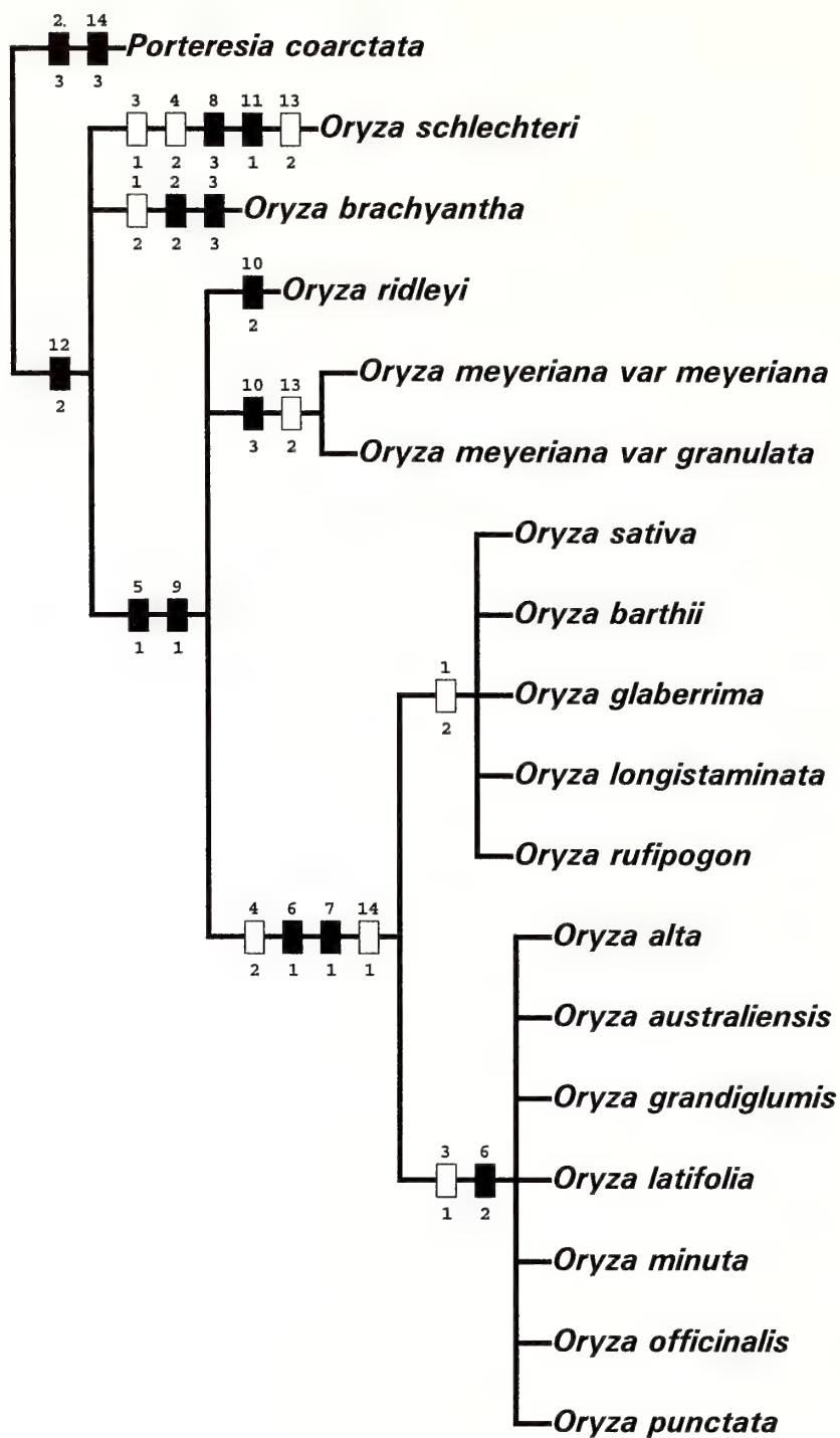
FIGURE 33.—One of 16 equally parsimonious trees (length=23 steps, CI excluding uninformative characters=0.78; RI=0.88) analyzing 16 species of Oryza with Porteressia as an outgroup. (Solid bars=unique origin of states (synapomorphies) and hollow bars=reversals or parallel states.)
