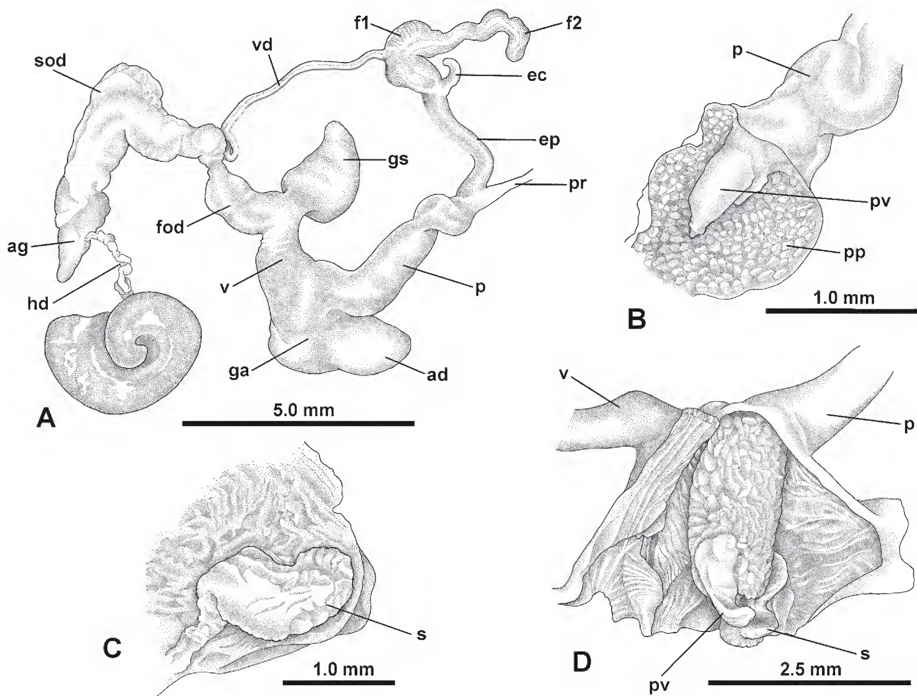
Fig. 16. Sheldonia wolkbergensis sp. nov., genitalia. A. Entire reproductive tract. B. Basal portion of penis opened to show penial verge. C. Atrial diverticulum dissected to show atrial stimulator. D. Partially everted distal genitalia with penis and stimulator protruding into genital atrium. A–C. Holotype (NMSA P0156/T4074). D. Paratype (NMSA W2258/T3168).
