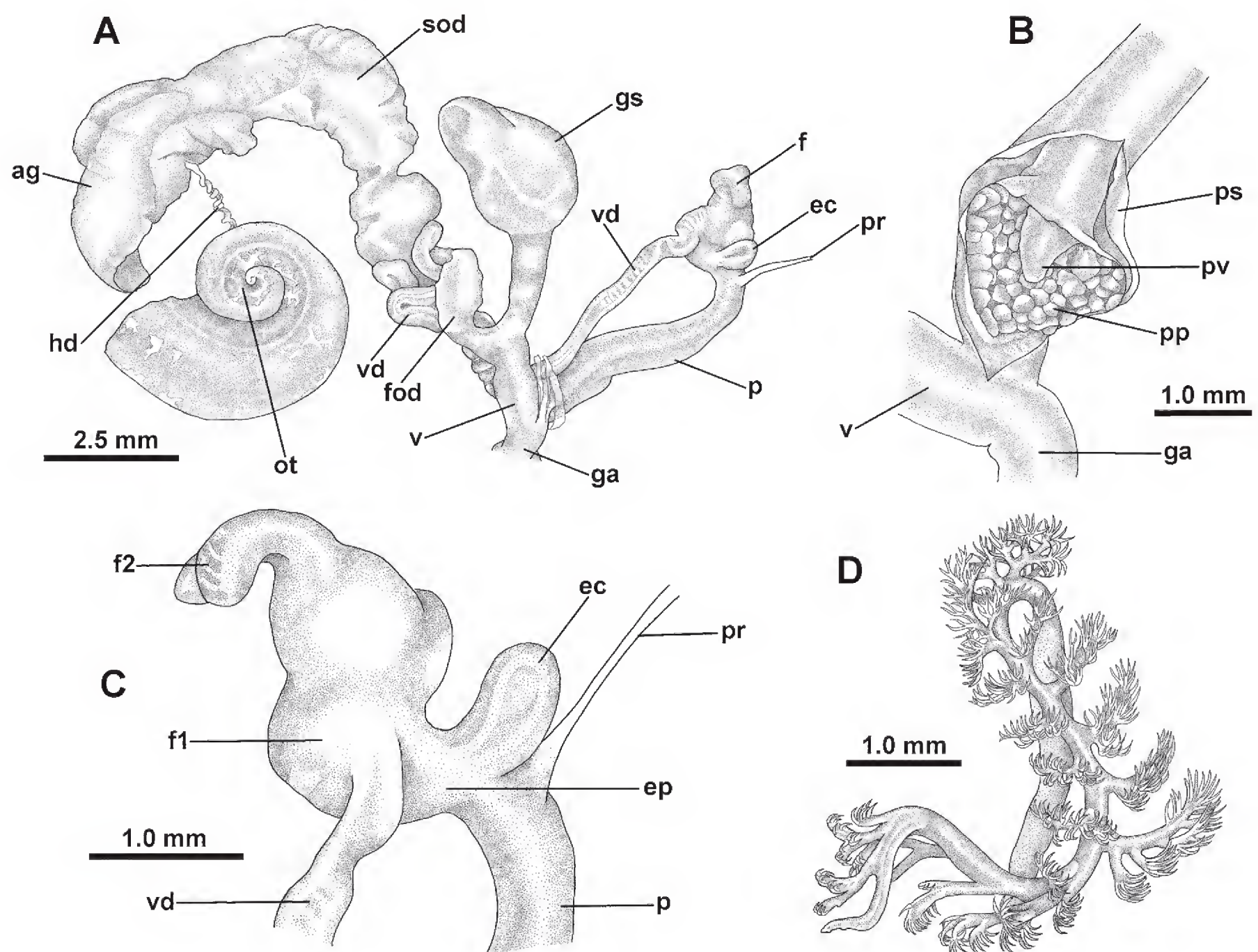
Fig. 7. Ptilototheca soutpansbergensis gen. et sp. nov., genitalia. A. Entire genital system. B. Basal portion of penis opened to show penial verge and coarsely papillate preputial region. C. Flagellum and epiphallus. D. Spermatophore. A–C. Paratype, NMSA P0304/T4060. D. Paratype, NMSA W2259/T4067.
