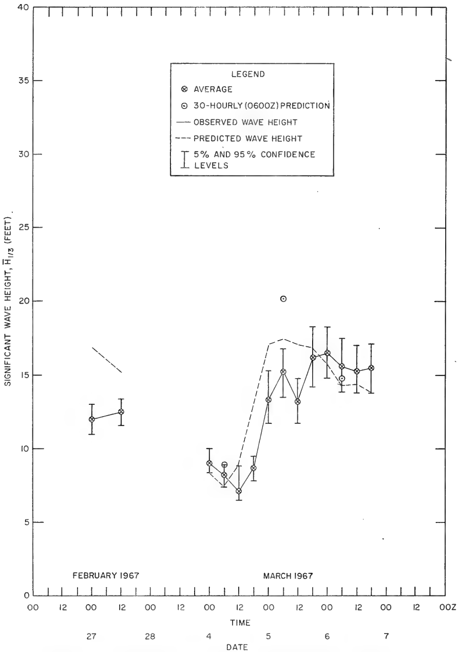
FIGURE 8. COMPARISON OF OBSERVED (MEASURED) AND PREDICTED WAVE HEIGHTS AT STATION K (FNWF WIND INPUT).
