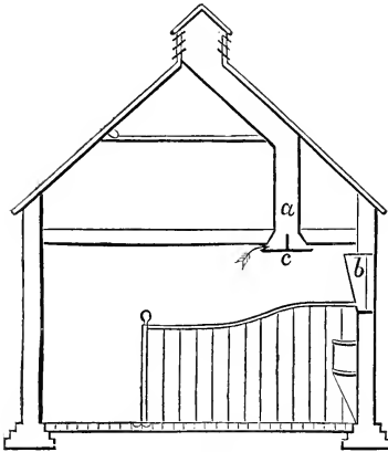
VENTILATING SHAFT.
