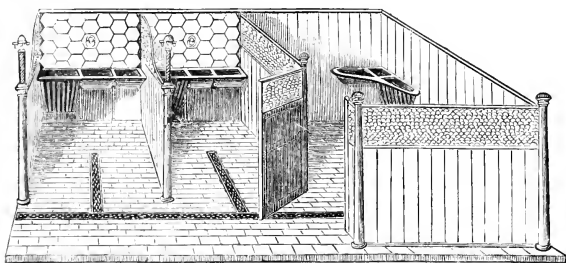
IRON FITTINGS FOR STALLS AND LOOSE BOX.
