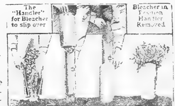
Celery Bleachers
