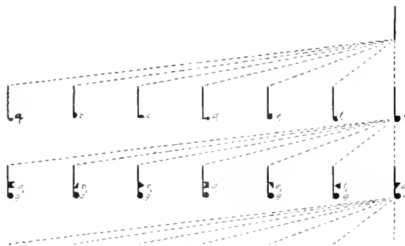
DIAGRAM 1. How Multiplication allows the origination of a beneficial combination of variations ( g_1 g_2 )
