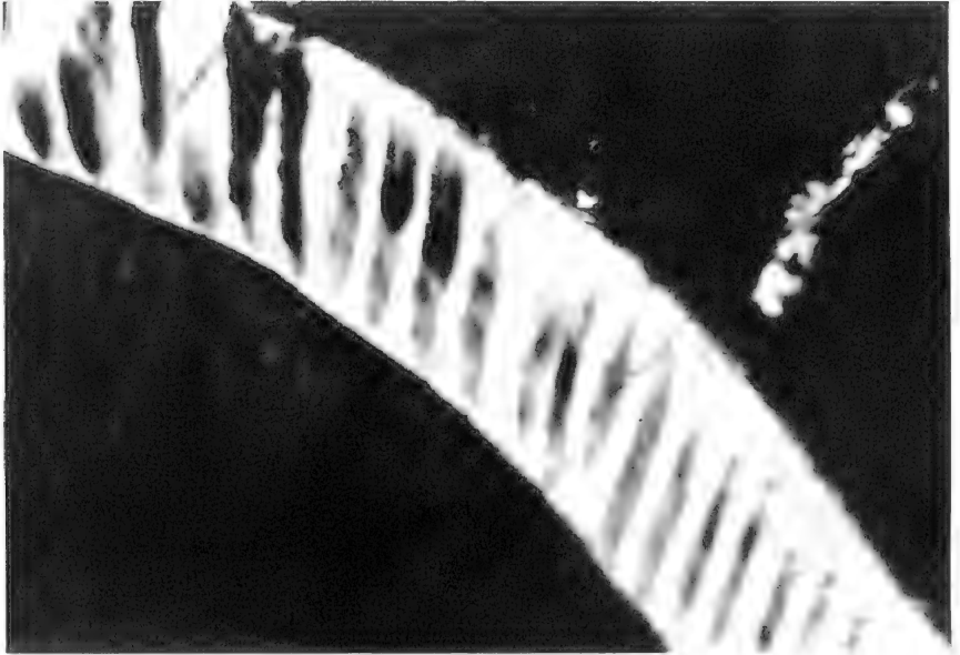
FIG. 15. The enamel of the late Cretaceous multituberculate Cimolodon (uncatalogued) demonstrates the typical banded appearance of continuous, non-prismatic enamel.
