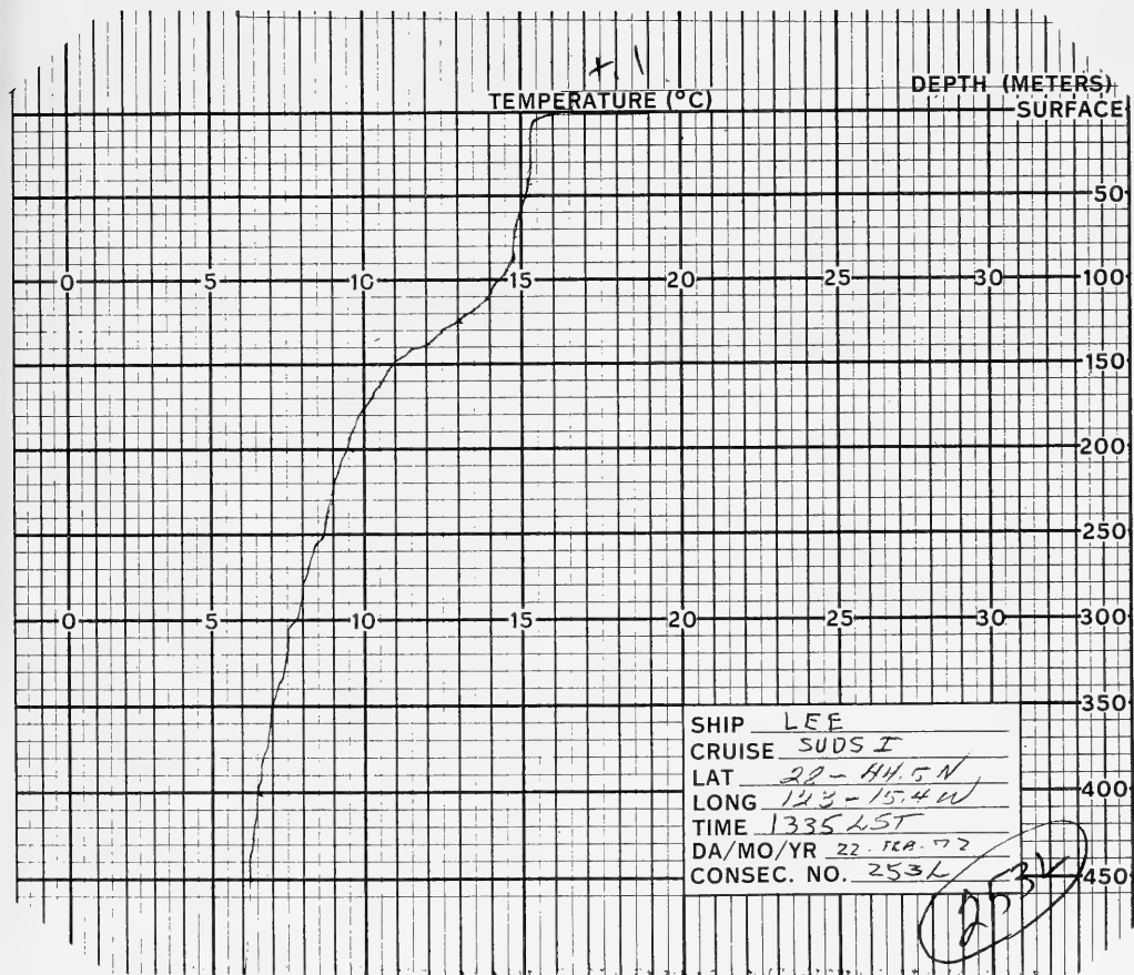
Figure 14b. SUDS I XBT 253L.
