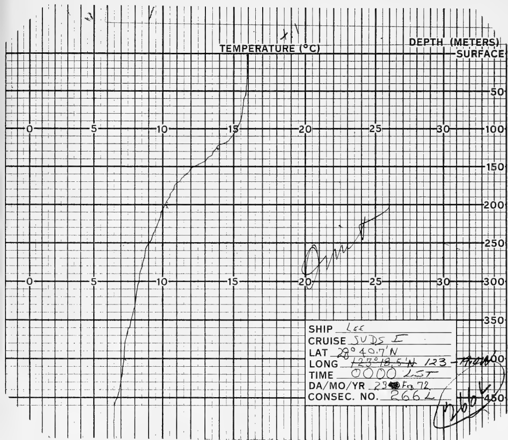
Figure 34. SUDS I XBT profile 266L.
