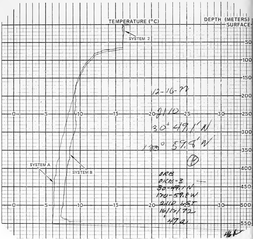
Figure 44a. Temperature profiles for ORB-3 XBT pair 46.
