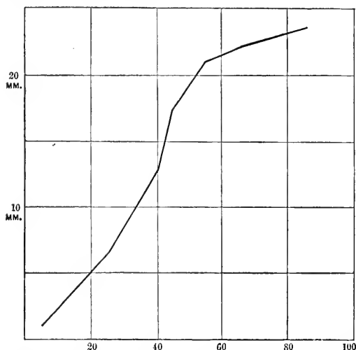
FIG. 80. — Curve of length of shell of Lymnaea stagnalis at intervals from hatching up to 85 days. From SENPER, Animal Life , p. 163.
