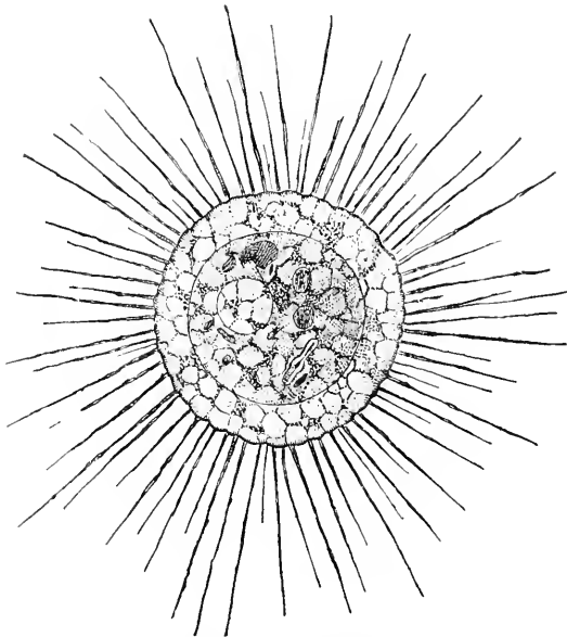
FIG. 17.— Actinospherium Eichhornii , unirritated. Natural size about 0.5 mm. (From VERWORN, '89.)
