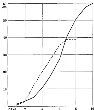
FIG. 82.—Curves of growth of Phaseolus multiflorus (continuous line) and Vicia faba (broken line). The ordinates represent actual lengths attained on the respective days by a bit of stem originally 1 mm. long. After SACHS, Lectures on Plant Physiology.
