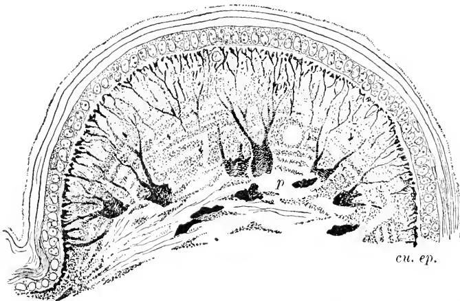
FIG. 57.—Vertical section through a black dermal papilla of Chamæleo vulgaris . ep , epidermis; cu , cutis; p , black pigment cells; p' , processes of the cells containing pigment; y' , yellow pigment cells. (After KELLER, '95.)
