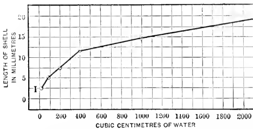
FIG. 134.—Curve of relation between length of shell of Limnæa stagnalis and quantity of water in which it is reared. (From SEMPER, '74.)
