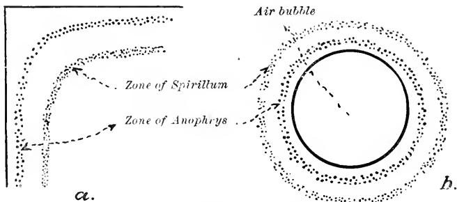
FIG. 2.— a. Corner of the glass slip covering a drop of liquid containing Spirillum and Anophrys , showing their aggregation with reference to the aerated bounding film of the drop. b. An air-bubble in the drop, showing aggregation of the organisms about it. (From MASSART, '91.)
