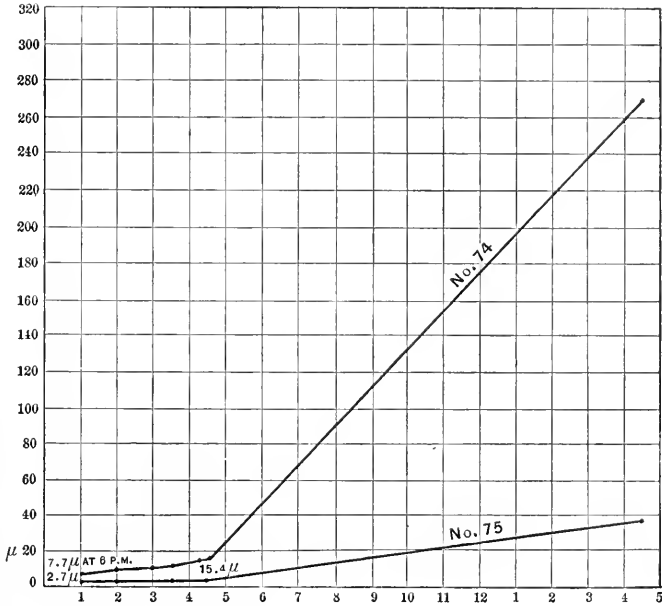
FIG. 123.—Curves of growth of threads of Bacillus ramosus in blue light (Experiment No. 75, of WARD) and in red light (Experiment No. 74). The numbers at the left indicate microns; at the bottom, hours. The retardation due to blue light is evident. (From WARD, '95.)
