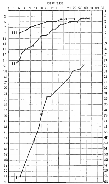
FIG. 67. — The mean thermal curves determined by ROSSBACH for the contractile vesicle of Infusoria. I, for Euplotes charon ; II, for Stylonychia pustulata ; III, for Chilodon cucullulus . The abscissæ indicate degrees of temperature, Centigrade, in two-degree intervals; the ordinates give the number of seconds elapsing between successive contractions of the vesicle, in two-second intervals. (From SEMPER, "Animal Life.")
