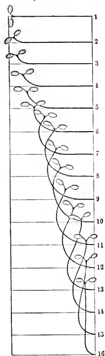
FIG. 108. — Course of geotropism in a plumule. The successive figures 1 to 16 indicate successive stages in the geotropic turning of a seedling growing in half darkness. Placed at first horizontal as at 1, the plant has become completely erect at 16. The most rapid growth is just behind the cotyledons and diminishes toward the base. The temporary bending beyond the vertical is to be noted. (From STRASBURGER, NOLL, SCHECK, and SCHIMPER, Textbook of Botany, Macmillan.)
