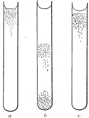
FIG. 24.—Glass tubes, about 0.5 cm. in diameter and 20 cm. long, fused at one end, and filled with water containing Paramecium (represented by points). a shows aggregation of the Paramecium at upper end of tube; b , aggregation of Paramecium around bacteria suspended in the water — chemotaxis veiling geotaxis; c shows that occasionally the Paramecia avoid the uppermost layer of the water. (From JENSEN, '93.)
