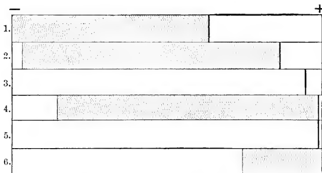
FIG. 56. — A diagram of MOORE'S photrum, showing for six spaces the epistrophic interval (shaded region). 1. Anacharis ( Elodea ) canadensis , "water-weed." 2. Lemna trisulea . 3. Saxifraga granulata (position of positive critical point). 4. Oxalis acetosella (position of negative critical point only approximate). 5. Pteris critica (positive critical point). 6. Pyrethrum sinense (garden Chrysanthemum ). + indicates the brighter end of the photrum.
