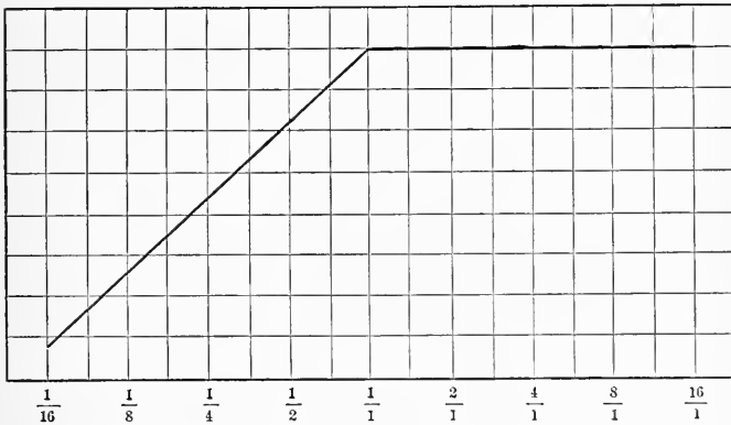
FIG. 44. — Curve showing the relation between intensity of light (abscissæ) and quantity of oxygen set free by Elodea canadensis . \frac{1}{16} indicates the unit intensity of the light from the heliostat. (From REINKE, '84.)
