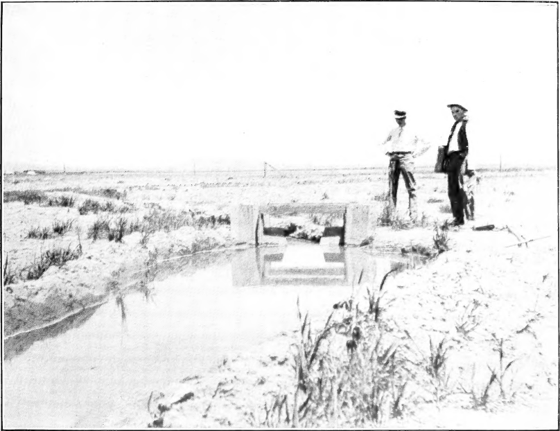
FIG. 1.—UPSTREAM VIEW OF CIPOLLETTI WEIR USED IN THE IDAHO INVESTIGATION.
