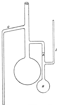
FIG. 1.—Apparatus for measuring the oxidation of soils.
