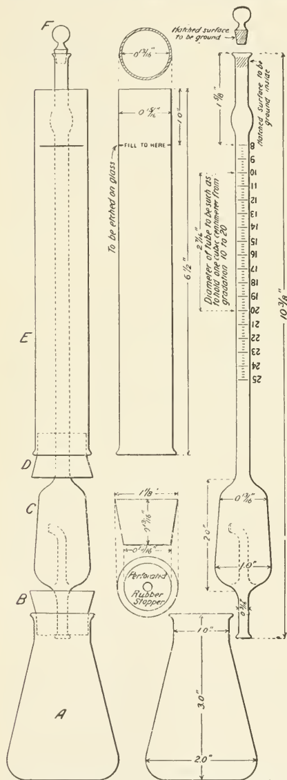
FIG. 1.—Apparatus for moisture determination.
