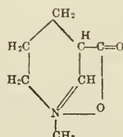
Arecain C_7H_{11}NO_2 .
