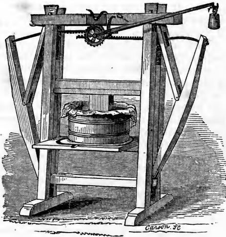
KENDALL'S CHEESE PRESS.
