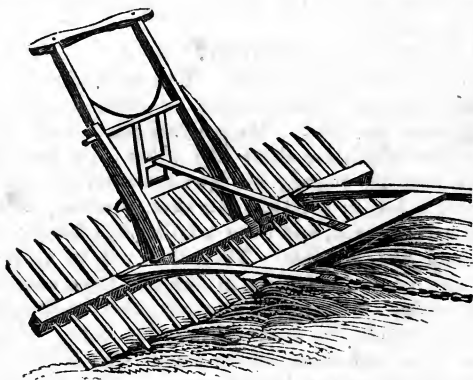
REVOLVING HORSE RAKE.
