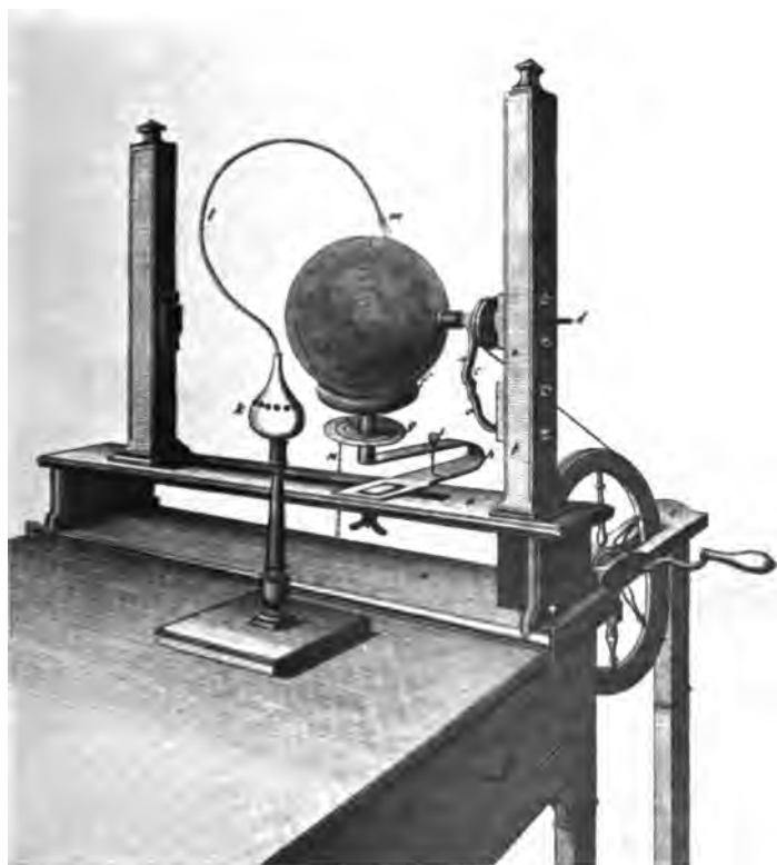
ELECTRICAL MACHINE AS USED BY PRIESTLEY, AND, PROBABLY, BY CAVENDISH.
