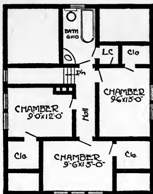
Figure 123.—Second Floor
