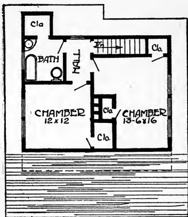
Figure 143.—Second Floor Plan
