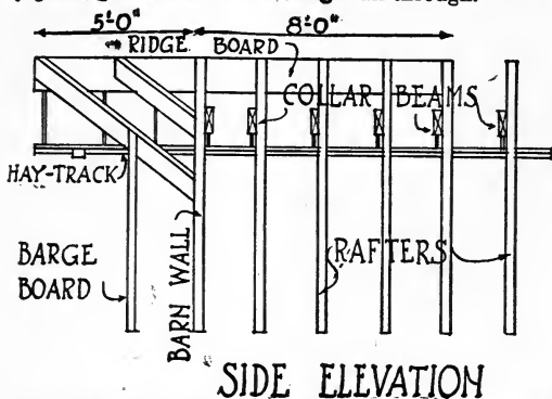
Figure 25.—Side View Showing Plan for Building a Hayfork Hood to Project from Peak of a Storage Barn. The Jack-Rafters form a Brace to Support the End of the Hay-Track Beam
