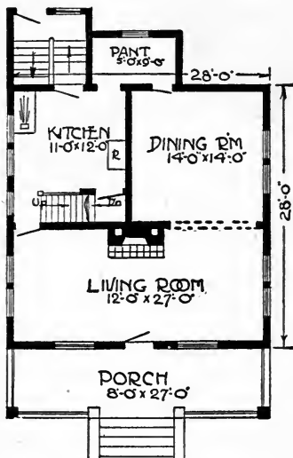
Figure 122.—First Floor
