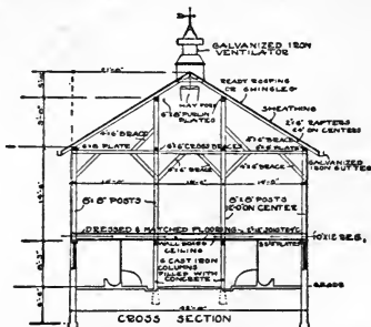
Figure 1.—Cross Section of Old Style Timber Frame Barn, 42 Feet in Width
