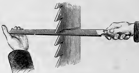
Fig. 101.—FILING UNDERNEATH.
