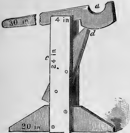
Fig. 124.—MICHIGAN WAGON JACK.
