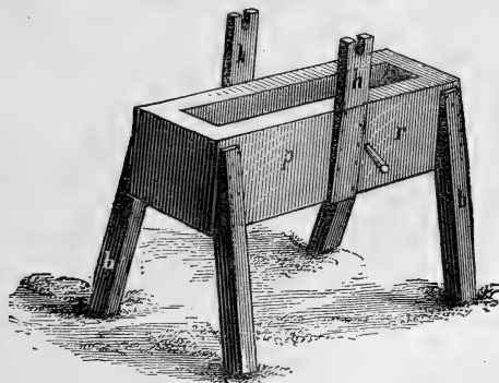
Fig. 175.—A BOX FOR A GRINDSTONE.
