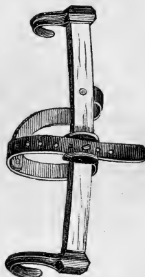
Fig. 117.—COW-FETHER.
