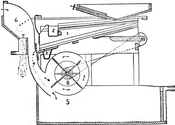
FIG. 22.—A hand power seed cleaner. The seed is sifted through screen as far as 1, the straw, particles, etc., being eliminated at 2. As the seeds slide down over the screen above 3, the sand and fine seeds drop through and are eliminated. The good seed passes into the air shaft at 4, the air moving upward forced by the rotary fan at 8. The perfect seeds being heavier fall and pass out at 5. The remaining dust, chaff, etc., are discharged through the dust hood at 6. Light, imperfect and foreign seeds fall into the opening at 7. (Courtesy A. T. Ferrell & Co., Saginaw, Michigan.)
