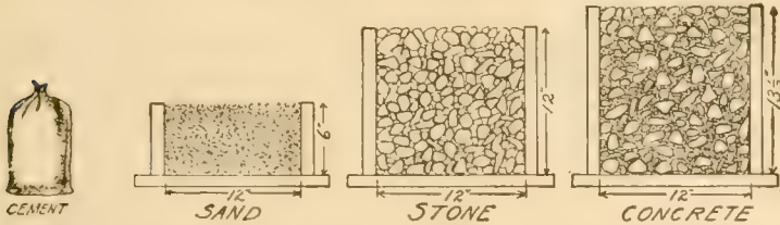
Fig. 1.—Quantities of cement, sand, and gravel in 1:2:4 concrete mixture, which means 1 part cement, 2 parts sand, 4 parts crushed stone or gravel, and the resulting quantity of concrete, which is only slightly greater in size than the gravel, the sand and cement filling the voids in the gravel.
