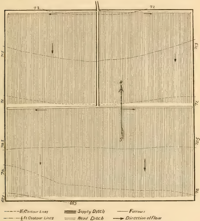
Fig. 15.—Method of Irrigating by Furrows.
