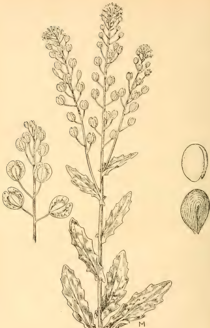
FIG. 3.—FRENCH-WEED.
