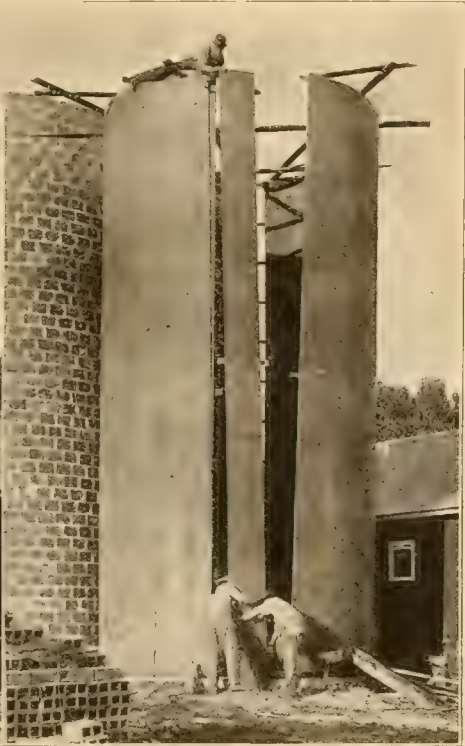
Fig. 12.—Erecting a Silo without scaffolding. Finished.
