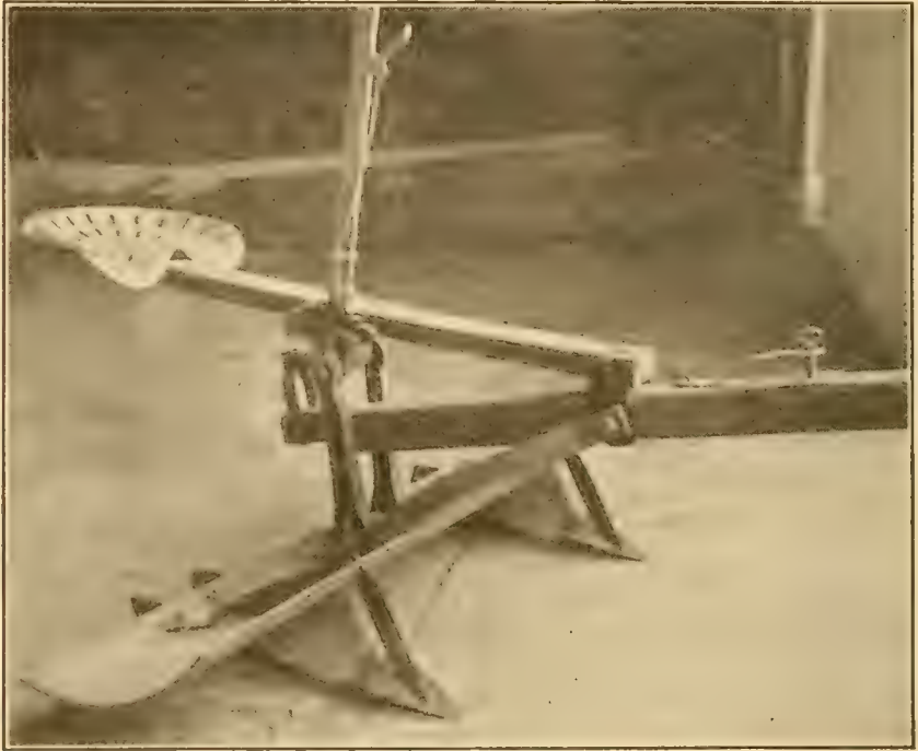
Fig. 16.—A Corrugator or Furrow Plow. This is used for making the small furrows or ditches when the furrow system of irrigation is used. The implement is adjustable both as to the depth and the spacing of the furrows.
