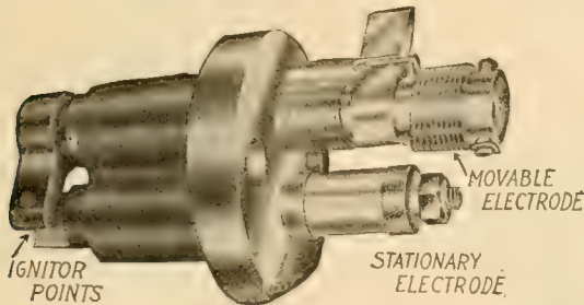
Fig. 3. Make-and-break Ignitor.
