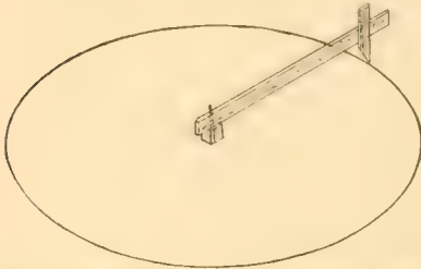
Fig. 3.—Laying Out Circle for Excavation a simple method of constructing a foundation and more practical than some that are more complicated.
