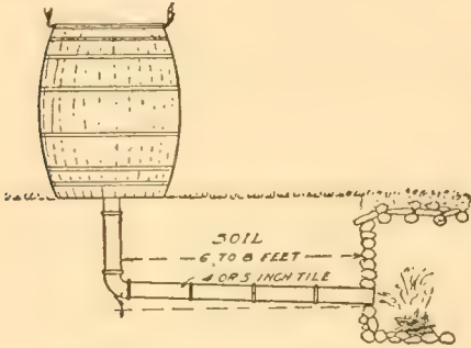
Fig. 10.—Cold Smoke Smokehouse.
