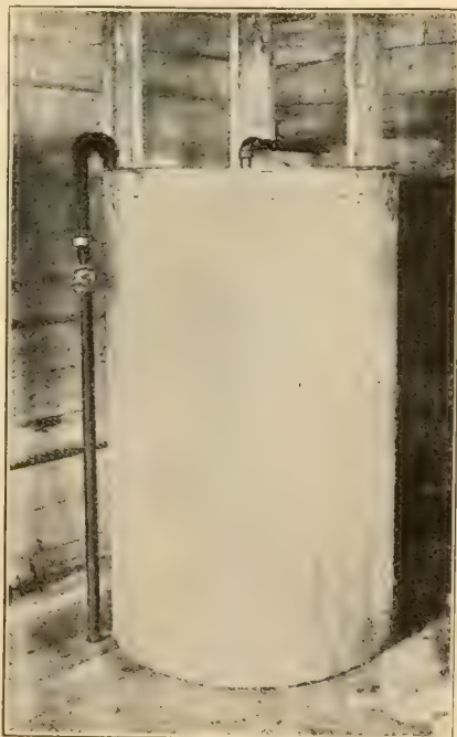
Fig. 2.—Tank used with steam heat. There is a steam coil in the bottom of the tank like the one shown on front page.
