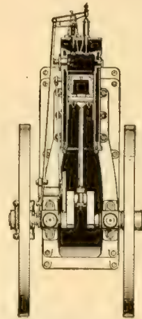
Fig. 7. Point of Ignition, near end of Second Stroke.
