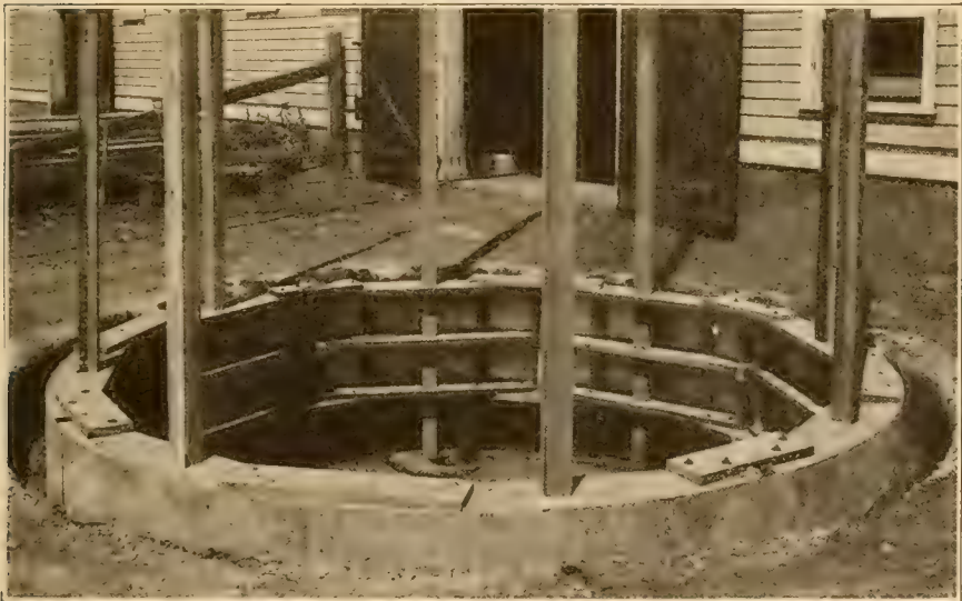
Fig. 36.—Two pieces of 2x4 are used to keep each section of the silo forms perfectly plumb. The inside form is shown here in position after the first filling. It is now ready for the second filling which should bring the concrete to the ground level.
