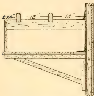
Fig. 6.—Hinged Perches and Dropping Board.
