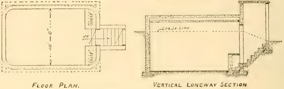
FLOOR PLAN.
