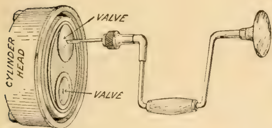
Fig. 13. Method of grinding valves.
