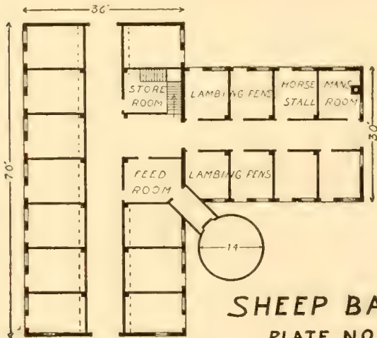
FLOOR PLAN SCALE IN FEET
