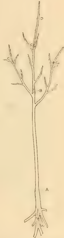
Fig. 7.—To be certain your trees are not too old, determine their age by counting their bud scars. The union of the stock and scion is shown at A; the end of the first year's growth at B; the end of the second year's growth at three points, C, C, C; and the three years' growth at D. A scale ring is shown at B.
