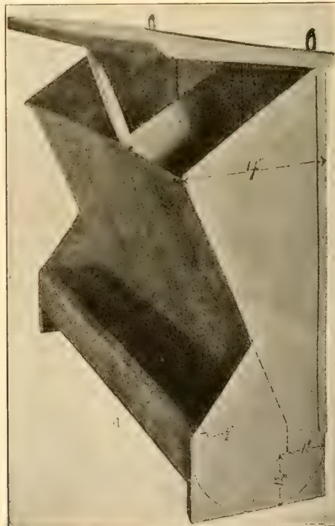
Fig. 12.—The End View of Grit Hopper, showing method of construction. Courtesy of the New York Experiment Station, Cornell.
