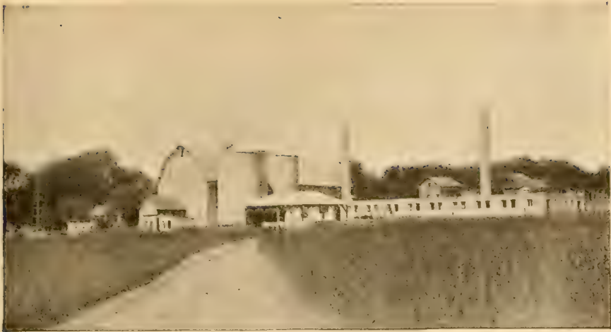
Concrete Dairy Barn, Hay Barn, Silos, Milk House and Manure Pit. The Dairy Barn is the Low Structure to the Right of the Illustration, and is Ventilated by Means of Two Concrete Stacks.
