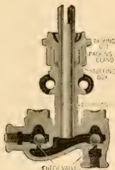
Fig. 15. Section of horizontal engine fuel pump.
