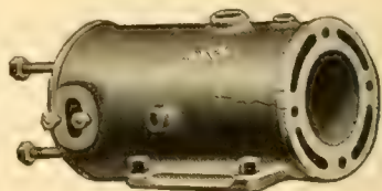
Fig. 19. Cracked Cylinder.
