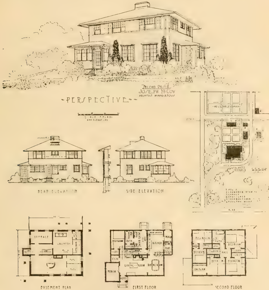
Fig. 5.—A House Designed for the Plains of the Middle West.
