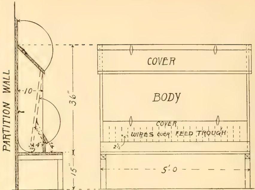
Fig. 11.—Working Plans of a Single Indoor Hooper. Courtesy of the New York Experiment Station, Cornell.
