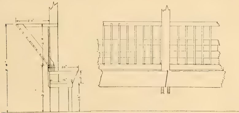
FIG. 4.—An Outdoor Feeding Rack.
