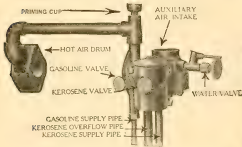
Fig. 16. Section of Horizontal Engine Kerosene Mixer.
