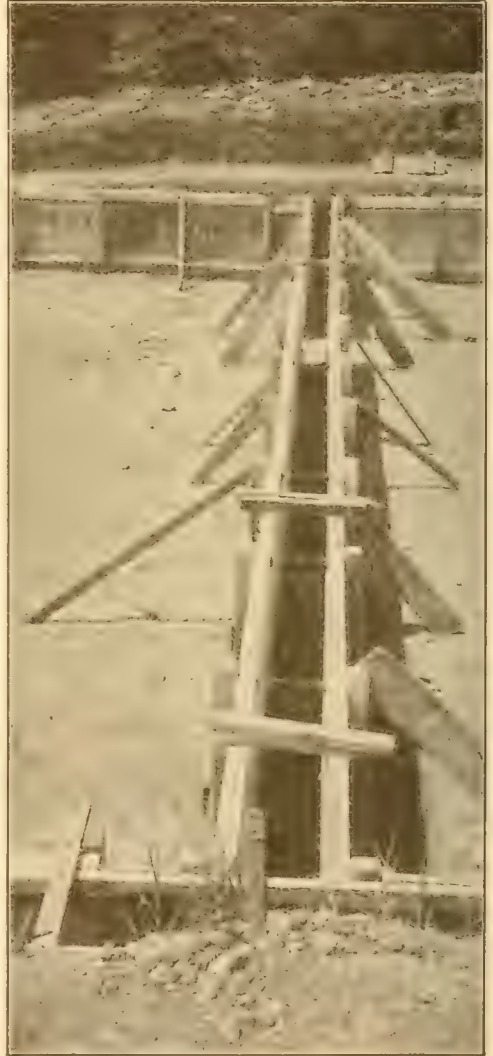
Fig. 12.—Wiring Forms Prevents Bulging.
