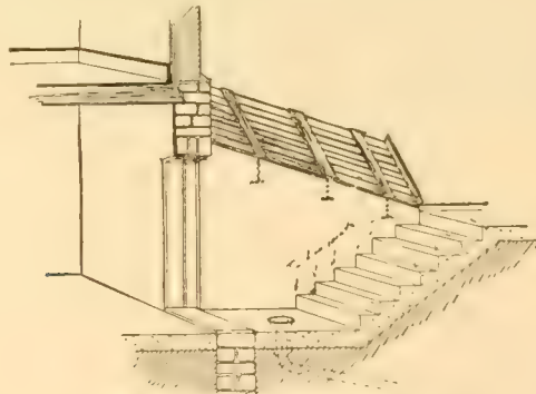
Fig. 40.—Diagram of Cellar Way.
