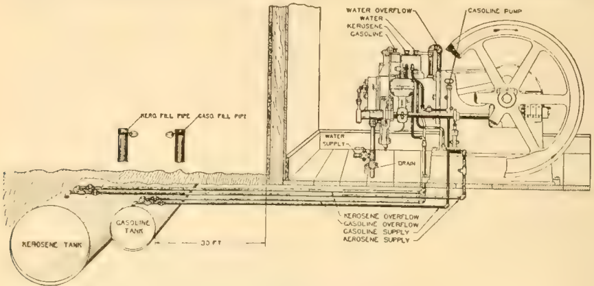
Fig. 3.—Showing location of engine with respect to fuel tanks.
