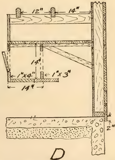
Fig. 7.—Different Types of Nests. A is a Tier of Nests with Broody Coop on Top. B and C Are Types of Wall Nests. D is a Nest Under the Dropping Board. Courtesy of the Wisconsin Experiment Station
