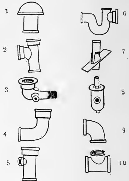
FIG. 348-a. Fittings for waste pipes:
