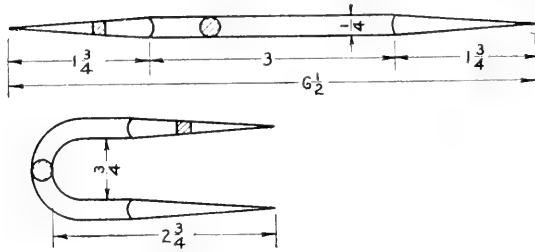
FIG. 176. Staple.
