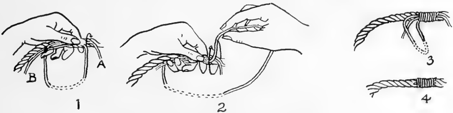
FIG. 363. Whipping end of rope.
