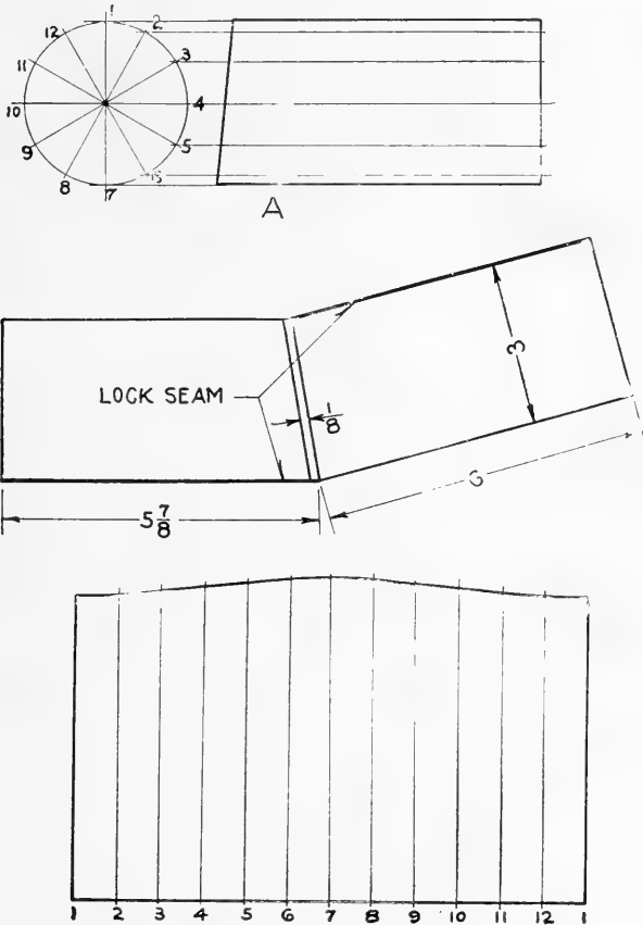
FIG. 295. Conductor elbow.
