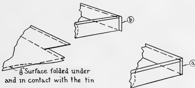
FIG. 272. Details of soldering watering pan.
