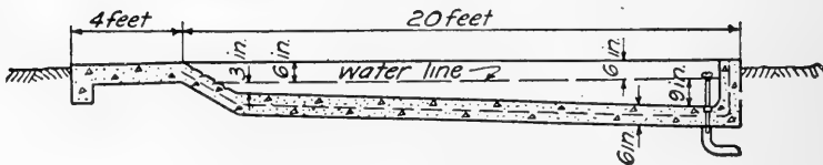
FIG. 170. Hog wallow.
