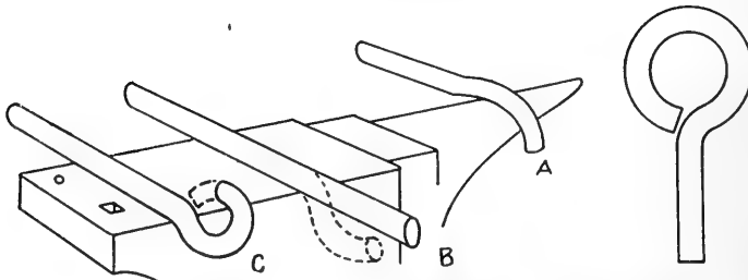
FIG. 179. Eyebolt, showing steps in construction.
