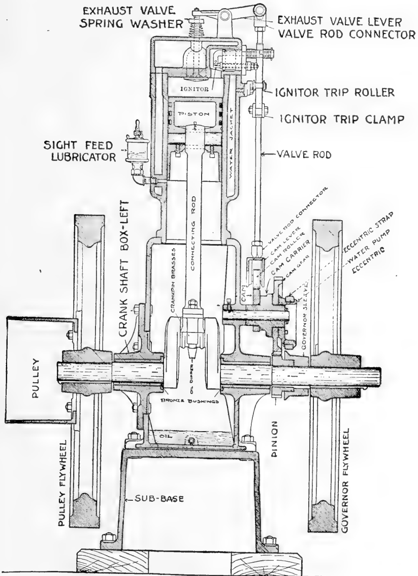
FIG. 326. Gasoline engine.
