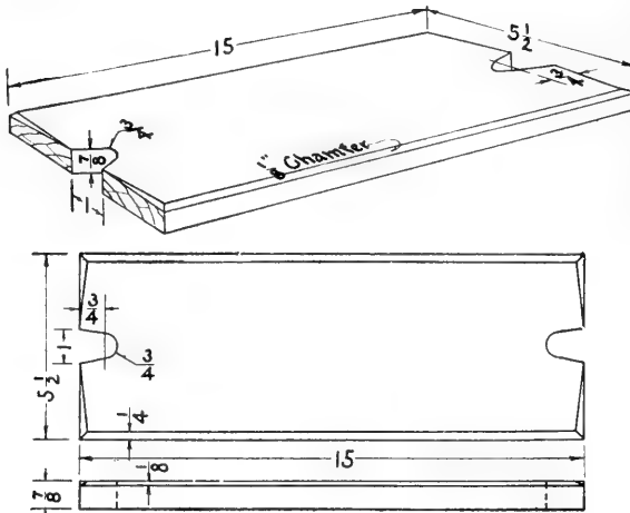
FIG. 50. Swing board.
