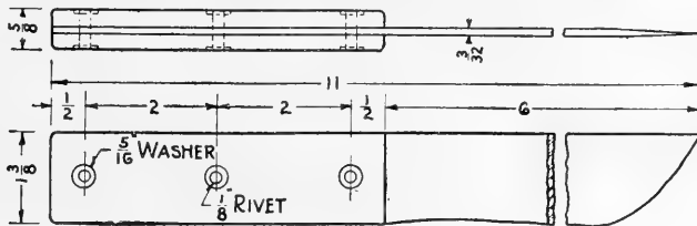
FIG. 221. Butcher knife.
