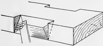
FIG. 105. Method of chiseling joints.
