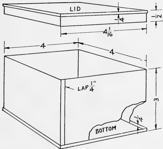
FIG. 293. Cubical box with lid.
