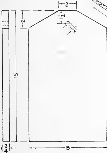
FIG. 47. Bread-cutting board.
