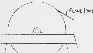
FIG. 53. Position of plane-iron on the grindstone.
