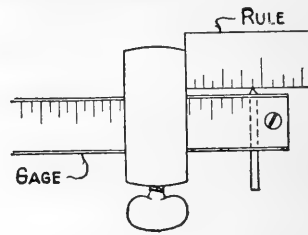
FIG. 24. Testing gage with rule.
