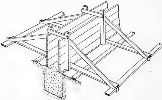
FIG. 152. Wall form above ground.
