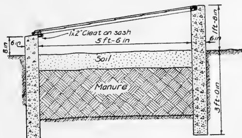
FIG. 150. Section thru hot-bed.
