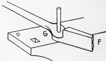
FIG. 245. Punching for rivet.
