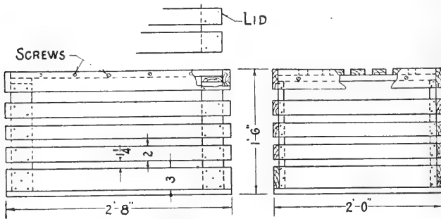
FIG. 74. Shipping crate.
