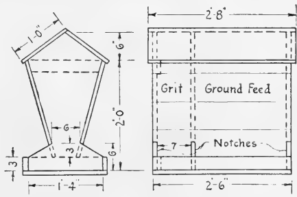
FIG. 128. Chicken feeder.
