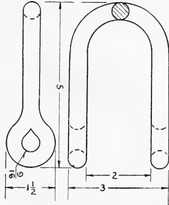
FIG. 206. Welded clevis.
