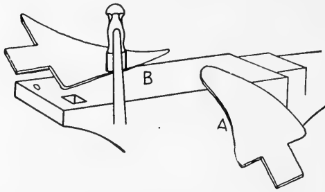
FIG. 226. Steps in sharpening cultivator shovel.
