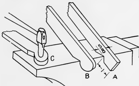
FIG. 201. Steps in making log hook.
