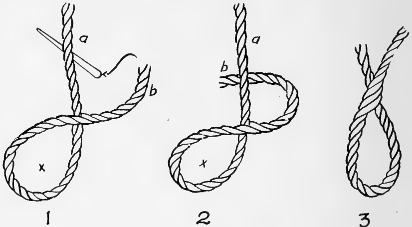
FIG. 395. Loop splice.
