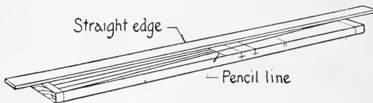
FIG. 31. Laying out rip-saw cuts.
