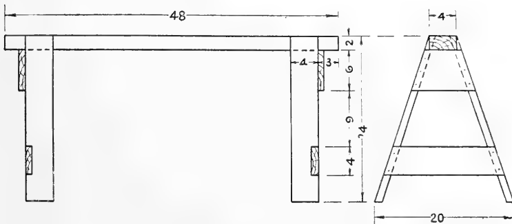
FIG. 88. Saw horse.
