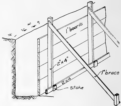
FIG. 151. Foundation wall form.
