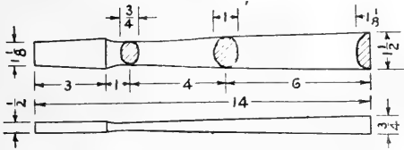
FIG. 110. Hammer handle.
