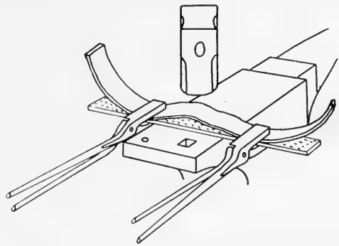
FIG. 258. Details of method of shortening tire.
