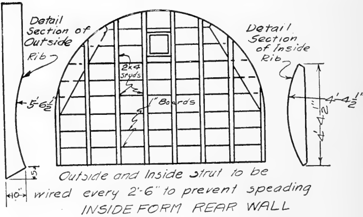
FIG. 169. Inside form of fruit storage cellar.
