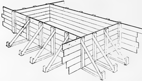
FIG. 166. Outside form for rectangular water tank.
