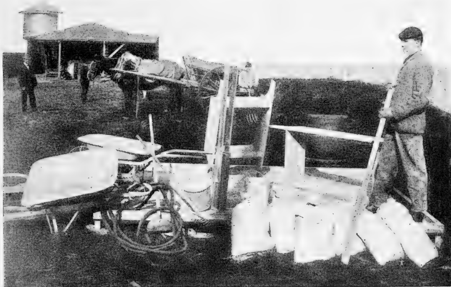
FIG. 145-a. Mixing concrete. Measuring boxes and other equipment.
