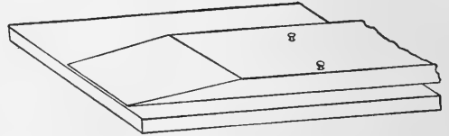
FIG. 328. Tapering for glue-joint.
