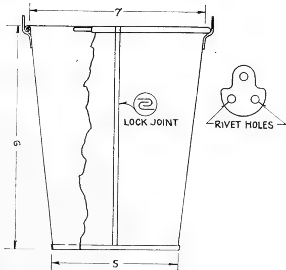
FIG. 288. Flaring pail.
