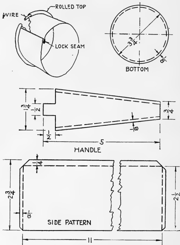
FIG. 285. Details of drinking cup.
