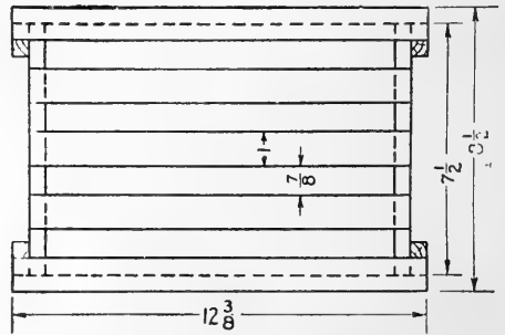
FIG. 14. Bottom of peck crate.
