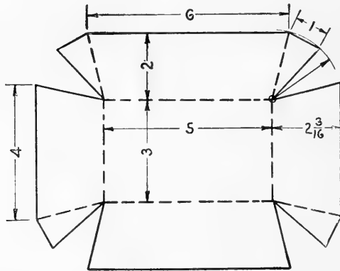
FIG. 275-a. Layout for drip pan.
