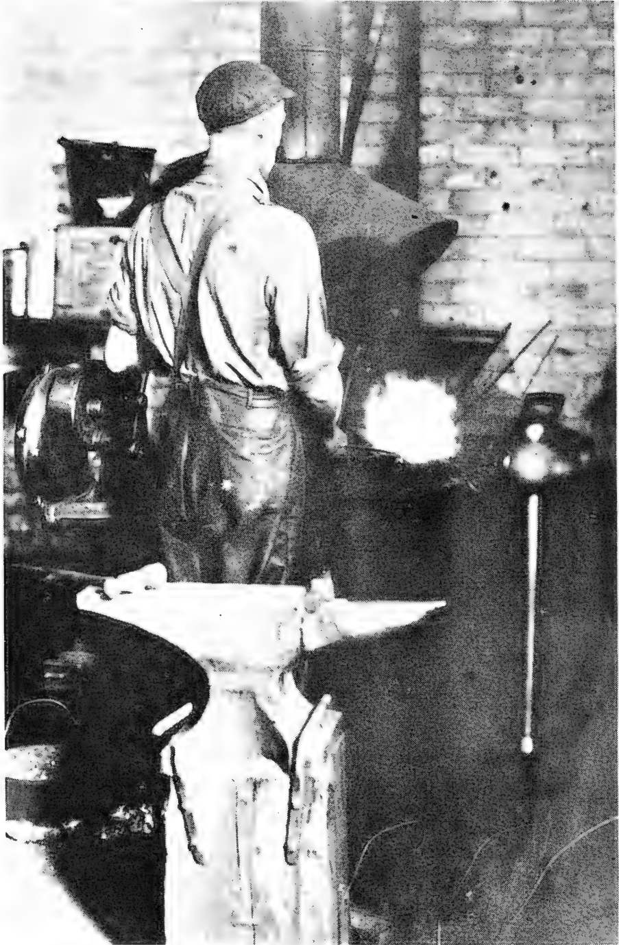
FIG. 172. Arrangement of forge and tools, showing position of blacksmith at the forge.
