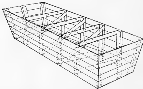
FIG. 167. Inside form for rectangular water tank.
