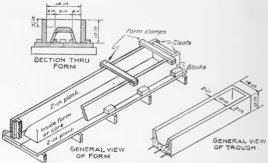
FIG. 158. Hog trough.
