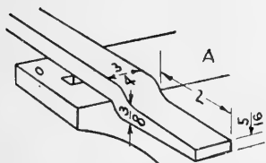
FIG. 240. Bending iron for forge tongs.
