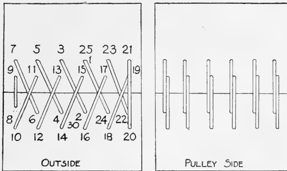
FIG. 334. Single-cross lacing; two rows of holes.
