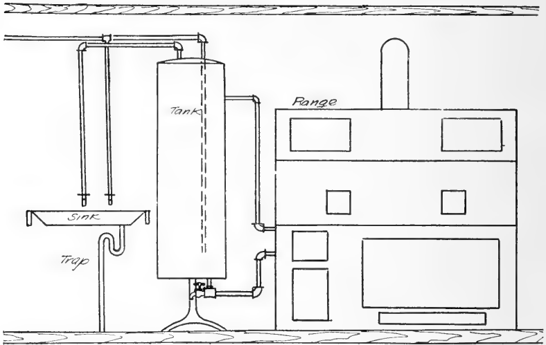
FIG. 357. A hot-water tank installation.
