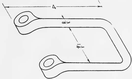
FIG. 196. Completed clevis.
