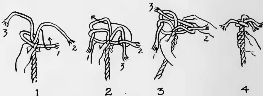
FIG. 365. Wall knot.
