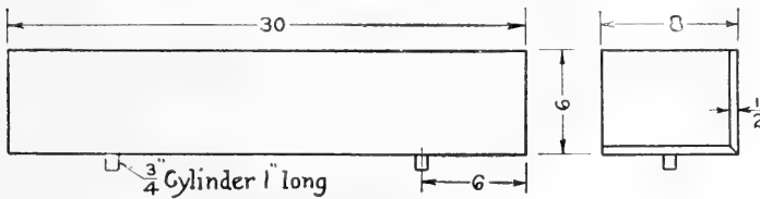
FIG. 274. Flower box.
