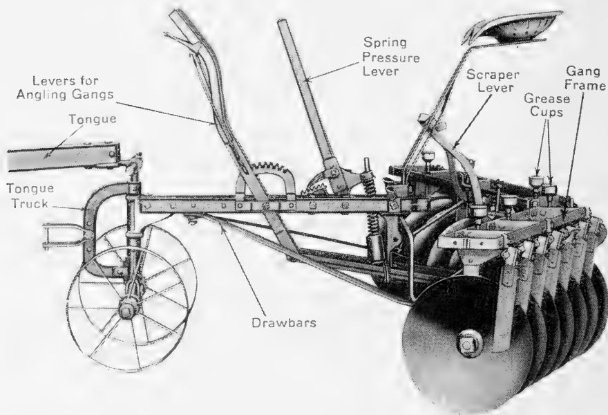
FIG. 318. Disc harrow.
