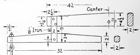
FIG. 132. Plow doubletree.
