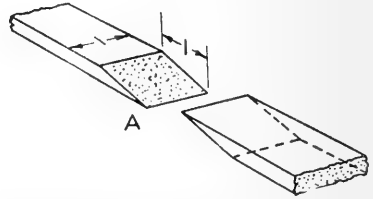
FIG. 230. Ends of metal prepared for welding.
