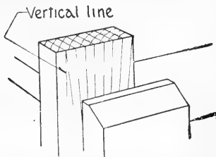
FIG. 37. Stock put in vise for rip-sawing.
