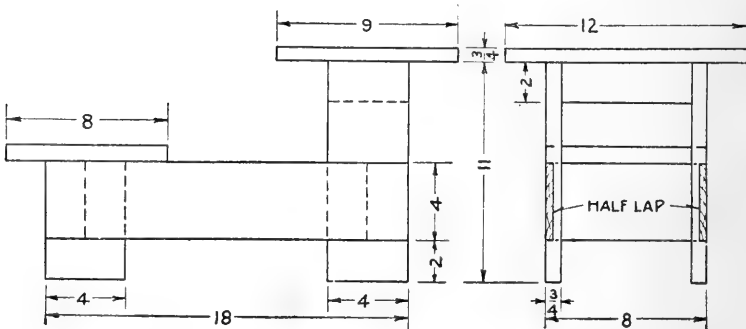
FIG. 84. Combination milk stool and pail rest.
