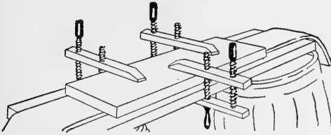
FIG. 330. A glue-joint in clamps.
