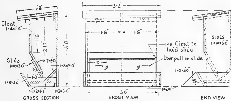
FIG. 122. Self-feeder.
