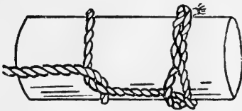
FIG. 389. Timber and half hitch.
