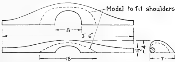
FIG. 114. Shoulder carrier.
