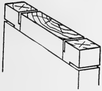
FIG. 97. Sawing the joints.
