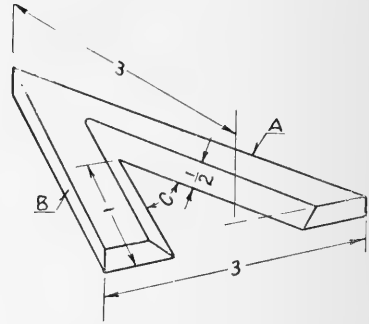
FIG. 249. New piece of stock for cultivator shovel.
