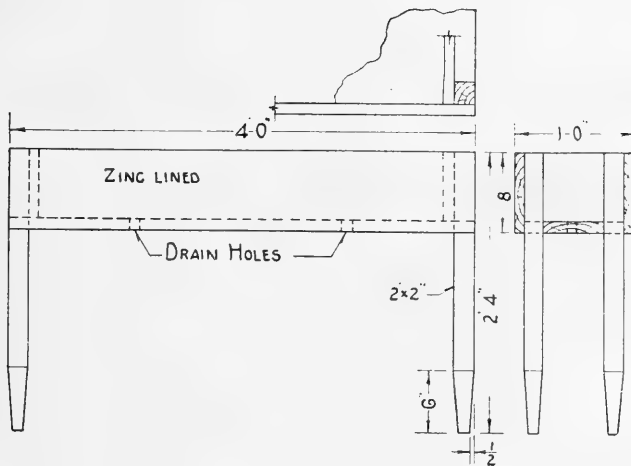
FIG. 75. Flower box.
