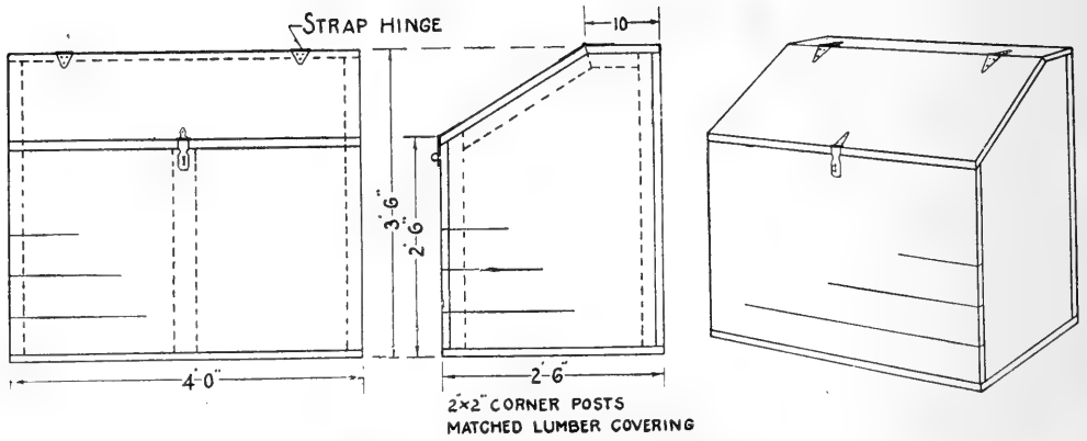
FIG. 73. Feed bin or wood box.
