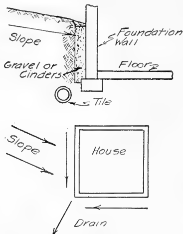
FIG. 360. Location of tile to drain house foundation.
