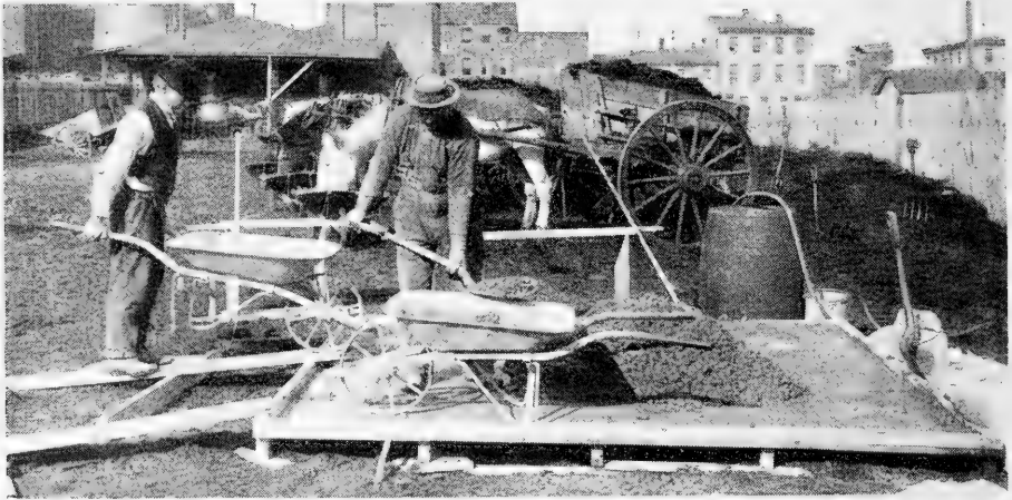
FIG. 142. Moving concrete with wheelbarrow.
