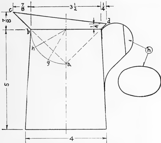
FIG. 298. A measure.
