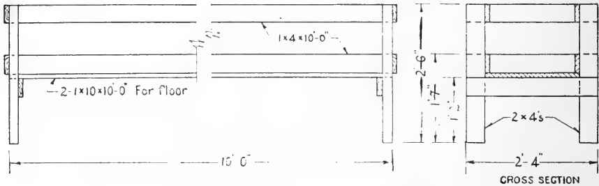
FIG. 131. Feed bunk for sheep.
