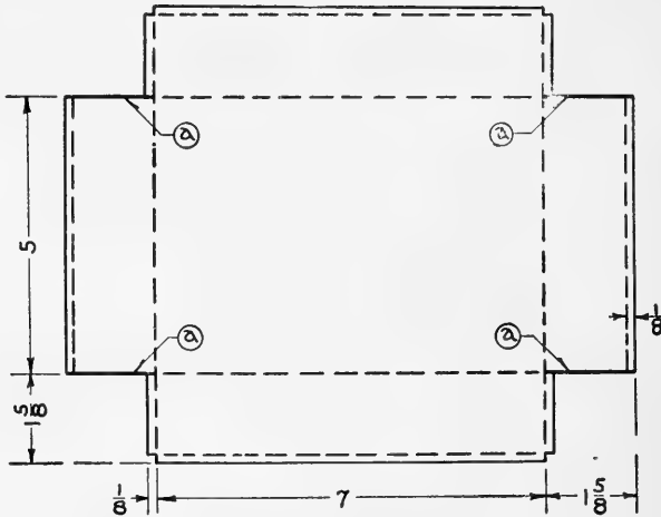
FIG. 271. Tin cut to shape for watering pan.
