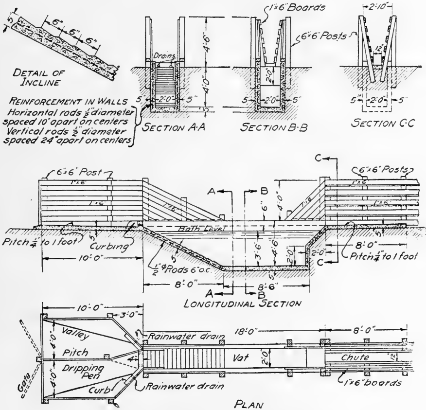
FIG. 171. Dipping vat for hogs.
