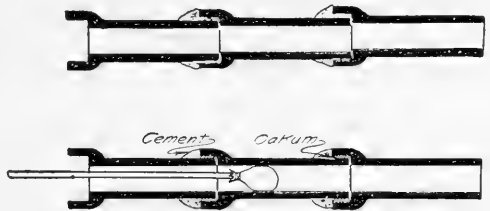
FIG. 352. Sewer tile made tight.
