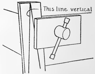
FIG. 38. Rip-sawing at an angle over the grain.
