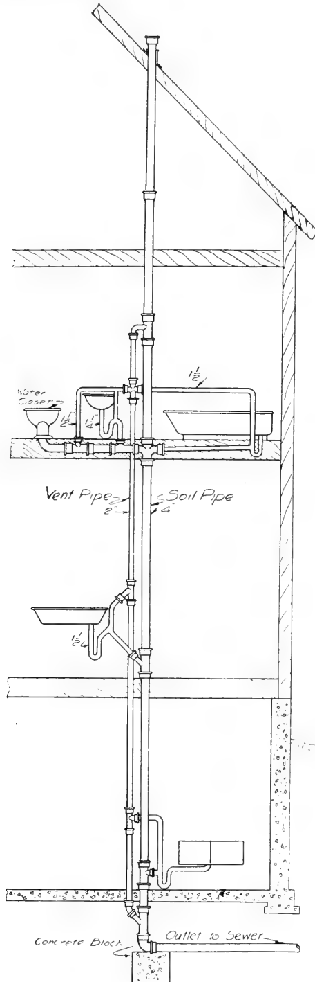
FIG. 354. Waste and ventilating pipe.
