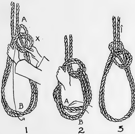
FIG. 381. Double rope bowline.
