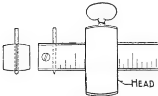
FIG. 25. Correct shape of point of marking gage.
