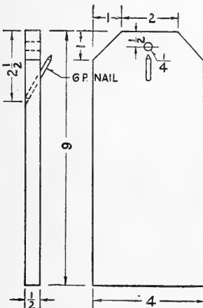
FIG. 47. Bread-cutting board.
