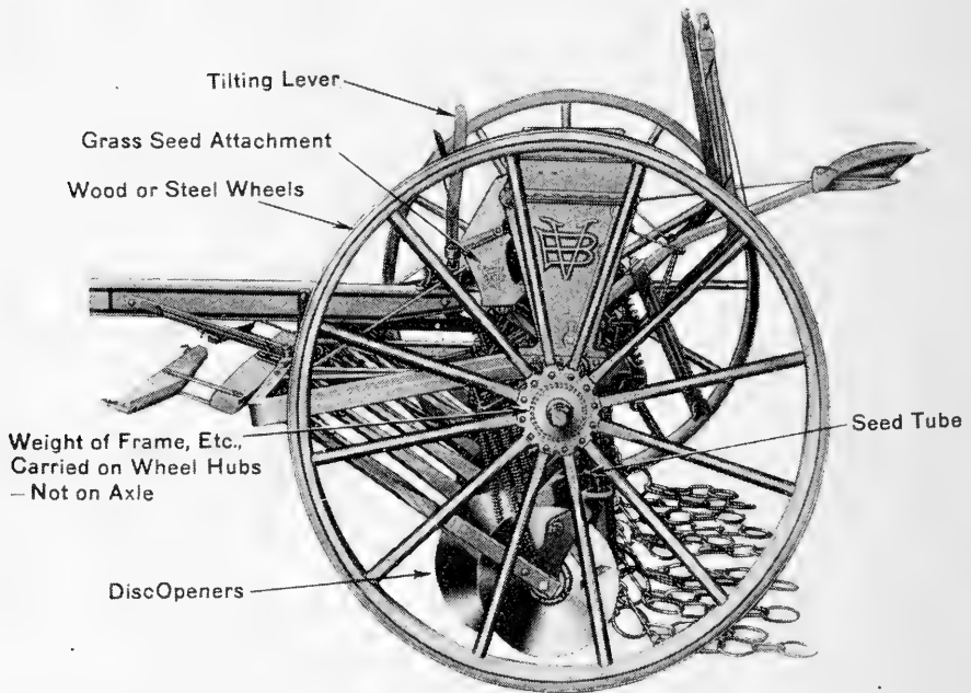
FIG. 319. Grain drill.
