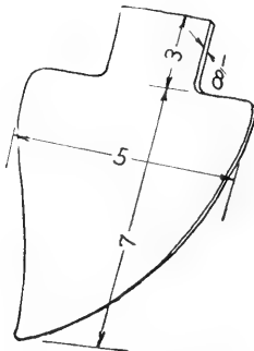
FIG. 224. Cultivator shovel.
