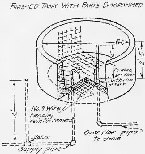
FIG. 155. Circular tank complete.
