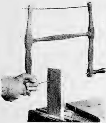
FIG. 115. Correct use of turning saw.
