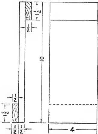
FIG. 46. Scouring board.
