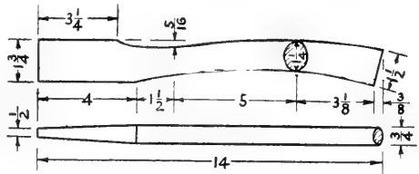
FIG. 111. Hatchet handle.
