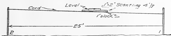
FIG. 350. Establishing a grade for tile.
