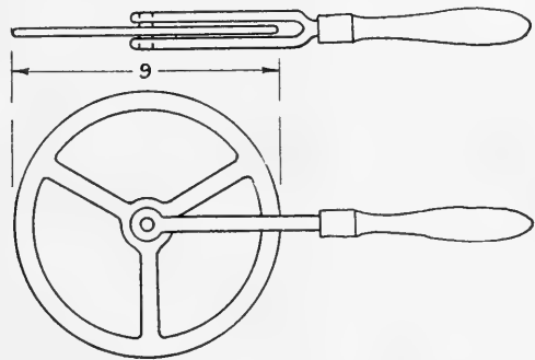
FIG. 259. Tire-measuring tool.
