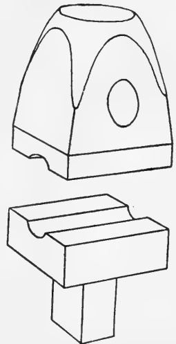
FIG. 247. Top and bottom swages.
