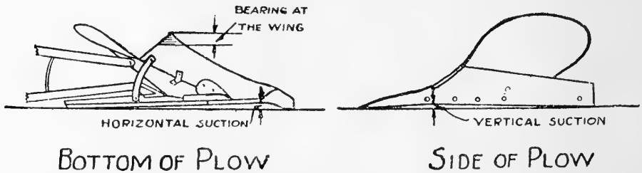
FIG. 315. Detail showing horizontal and vertical suction.
