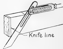
FIG. 43. Laying out with bevel square.
