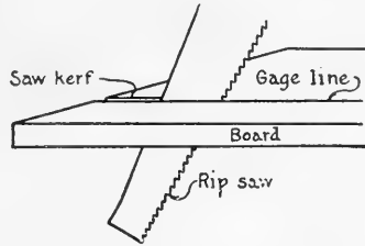
FIG. 16. Position of rip-saw in action.
