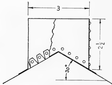
FIG. 296. Roof ridge flange.
