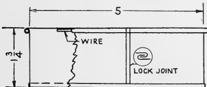
FIG. 280. Cylindrical pan.
