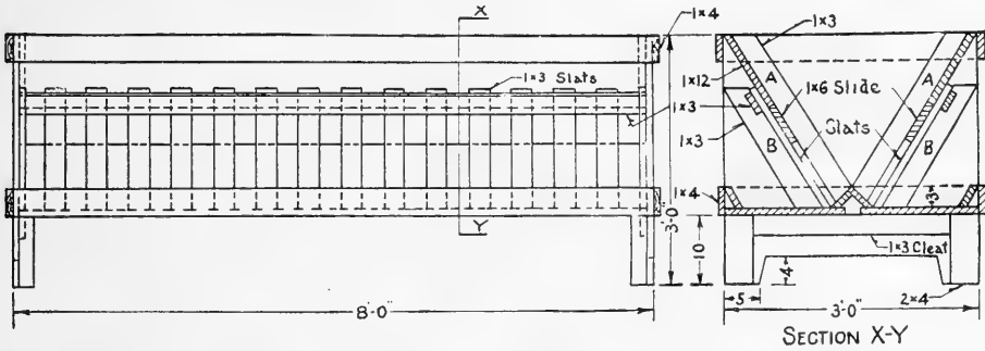
FIG. 118. Sheep rack and feed bunk.
