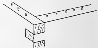
FIG. 103. Location of nails for stringing.
