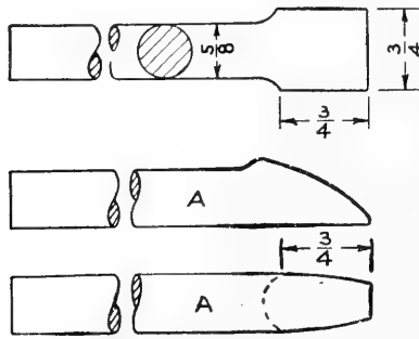
FIG. 203. Two-piece weld.
