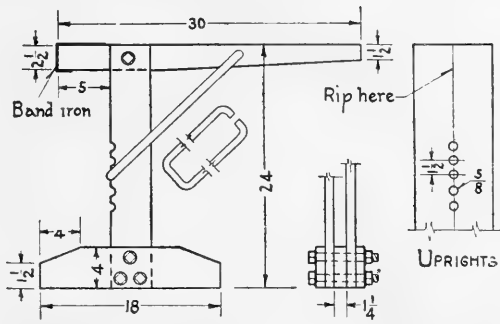
FIG. 134. Another type of wagon jack.
