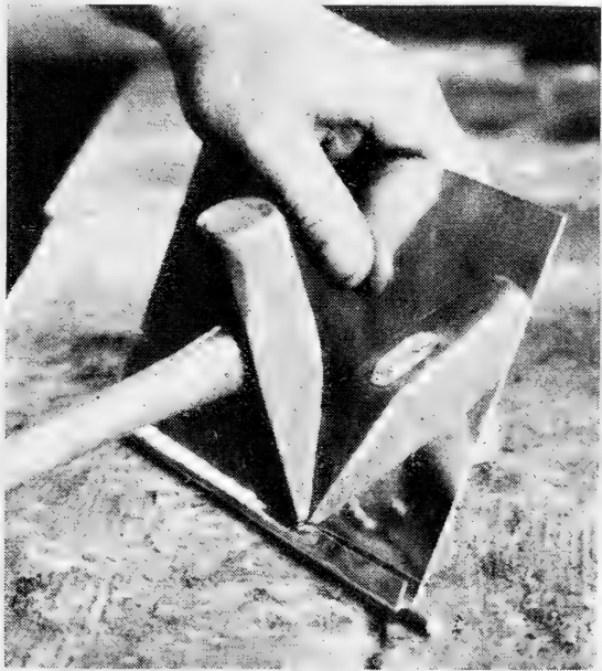
FIG. 284. Folding metal over wire.
