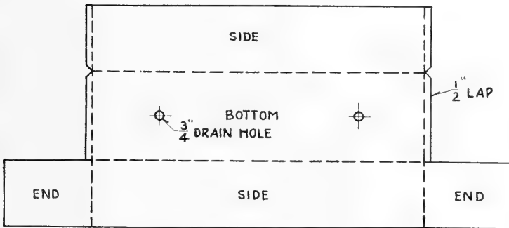
FIG. 274-a. Details of flower box.
