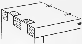
FIG. 93. Corner joint for seed tester.
