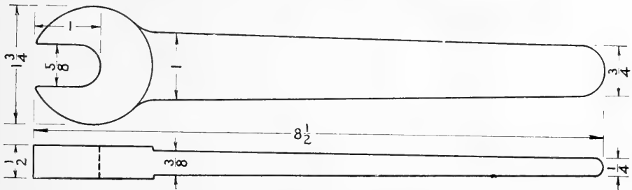
FIG. 186. Open-end wrench.
