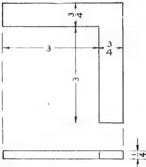
FIG. 237. Right-angle weld.
