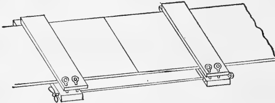
FIG. 329. Belt clamped for gluing.
