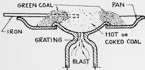
FIG. 175. Cross-section of forge.
