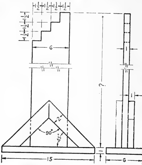
FIG. 11. Buggy axle rest.
