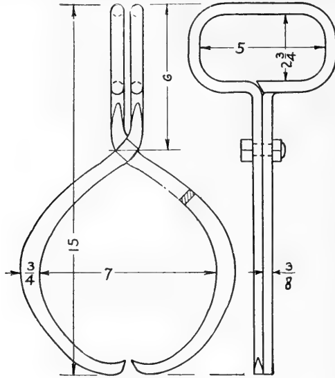
FIG. 236. Ice tongs.
