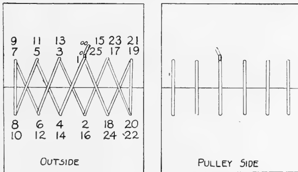
FIG. 332. Single-cross lacing; one row of holes.
