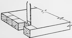
FIG. 99. Finishing the chisel cut.
