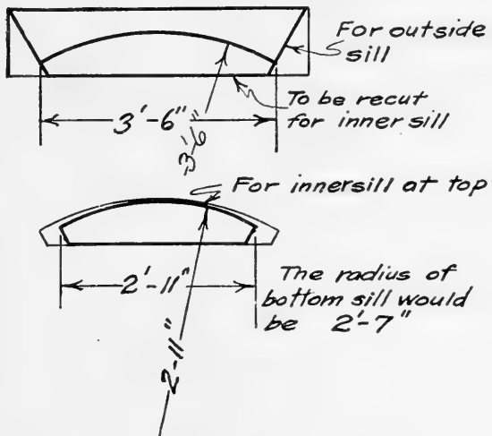
FIG. 154-a. Detail of sill for circular form.
