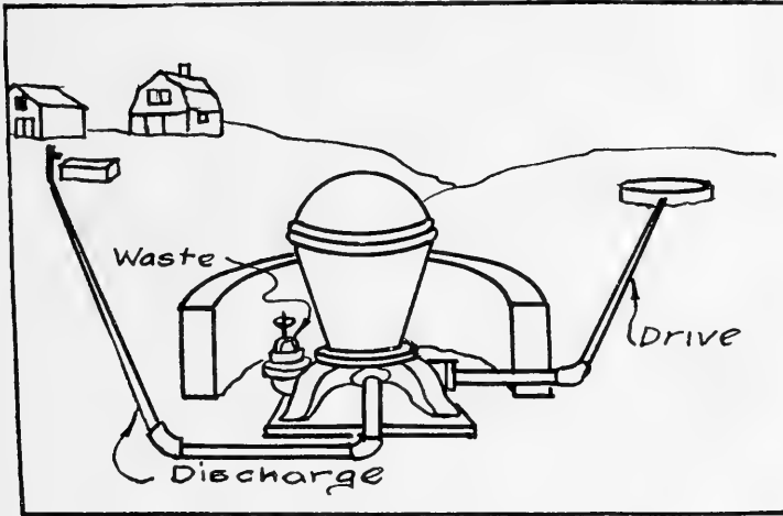
FIG. 359. Hydraulic ram.
