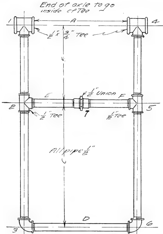
FIG. 349. Pipe handle for garden roller.
