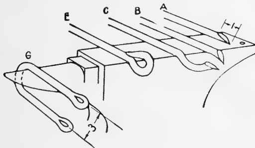
FIG. 216. Operations in making welded clevis.
