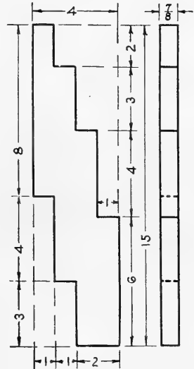
FIG. 10. Window stick.
