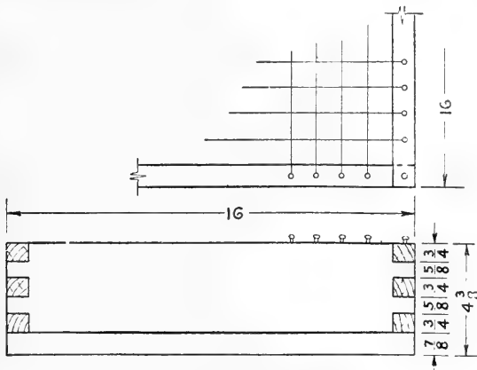
FIG. 87. Seed tester.
