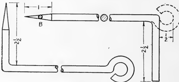
FIG. 183. Steps in making gate hook.
