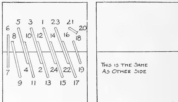
FIG. 336. The Annan lacing.
