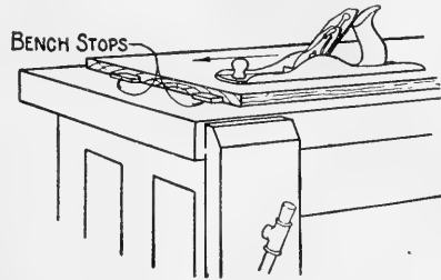
FIG. 60. Planing a wide board.
