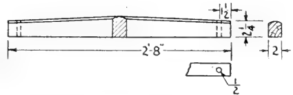
FIG. 113. Singletree.
