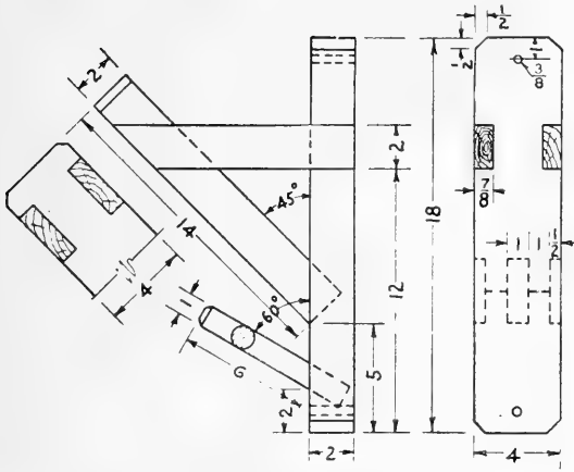
FIG. 85. Harness rack.
