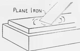
FIG. 54. Position of plane-iron on the oilstone.
