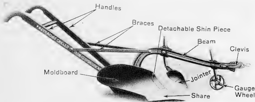
FIG. 314. Walking plow.
