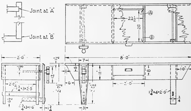
FIG. 119. Woodworking bench.
