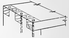
FIG. 100. Position of nails in joints.
