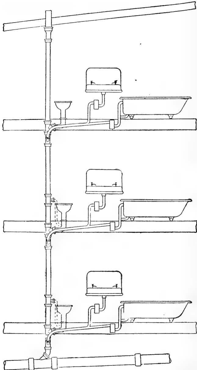
FIG. 354-a. Waste pipe without ventilating pipe.
