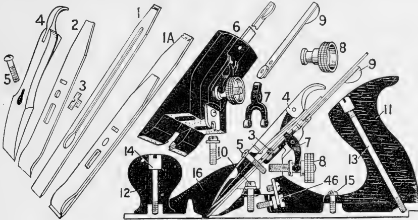
FIG. 52. Parts of jack plane:
