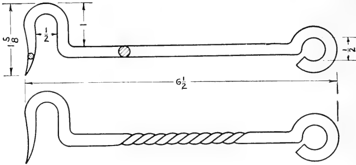
FIG. 177. Gate hook.
