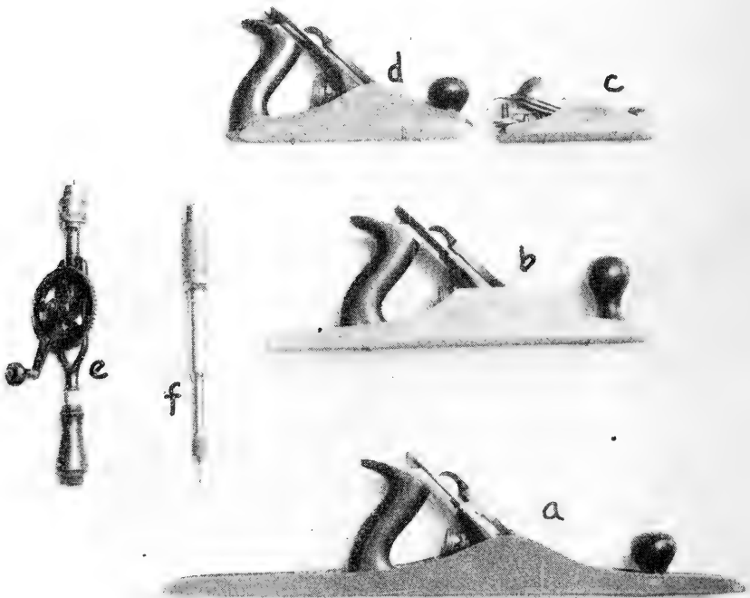
FIG. 3. a , jointer plane; b , jack plane; c , block plane; d , smooth plane; e , hand drill; f , automatic drill.
