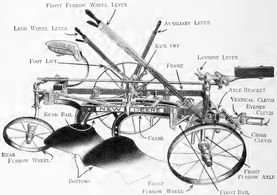
FIG. 316. Gang plow.
