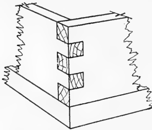
FIG. 101. Method of attaching the bottom.
