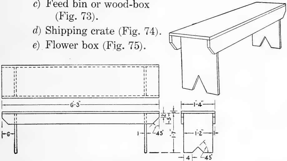
FIG. 71. Wash bench.
