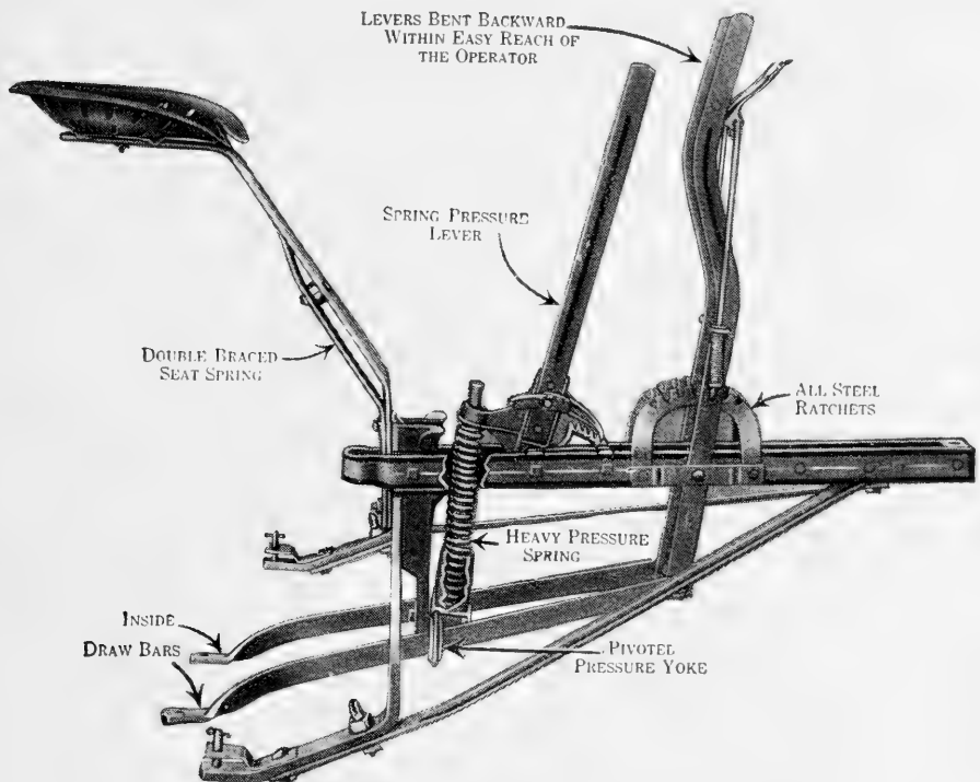
FIG. 318-a. Details of construction of disc harrow.
