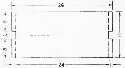
FIG. 276. Layout for watering trough:
