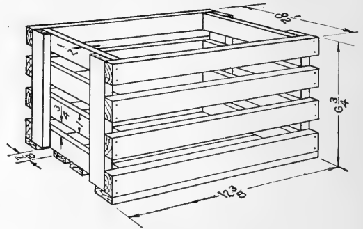
FIG. 12. Peck crate.
