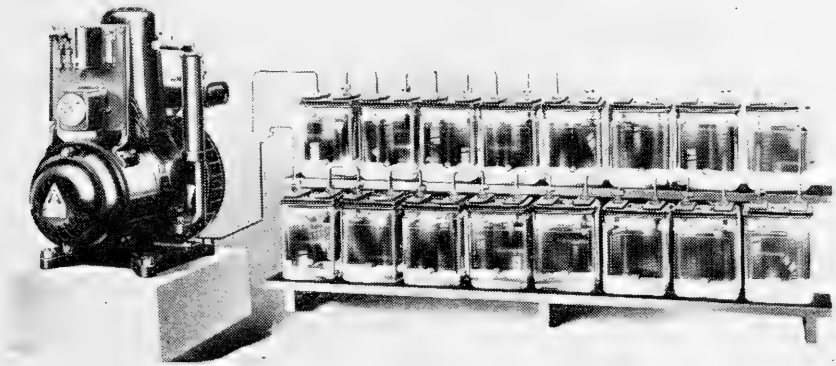
FIG. 312-a Farm lighting plant with storage battery.
