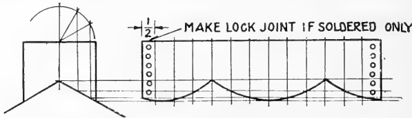
FIG. 297. Details of roof flange.
