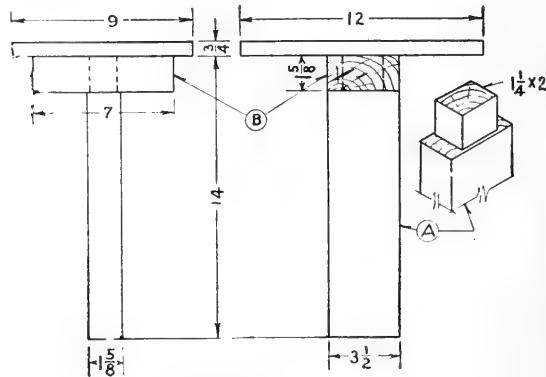
FIG. 83. Milk stool.
