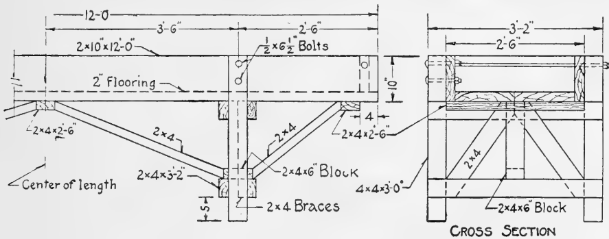
FIG. 126. Feed bunk for cattle.
