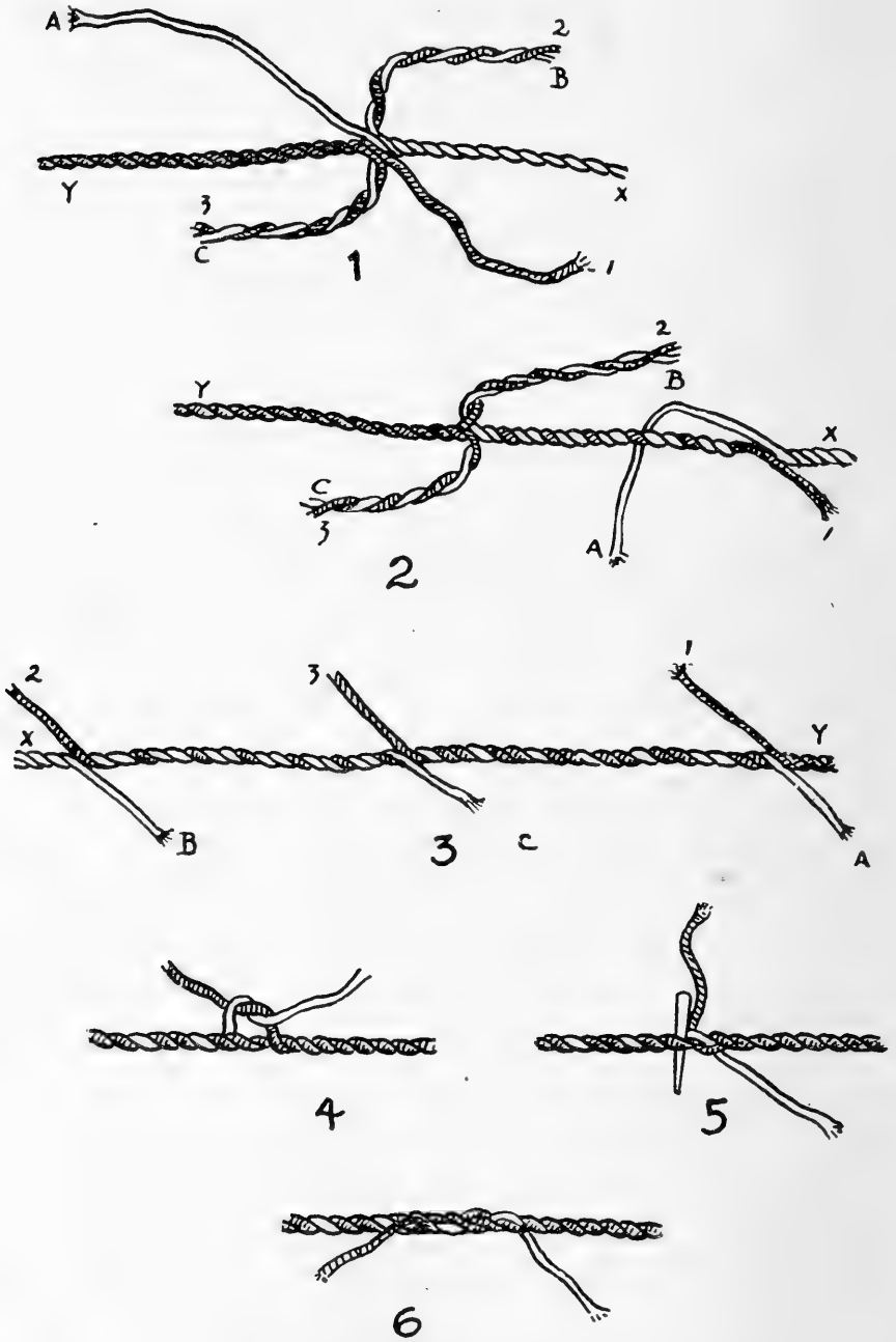
FIG. 398. Long splice.
