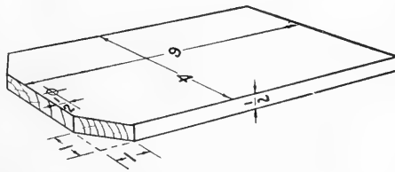
FIG. 49. Bill board.
