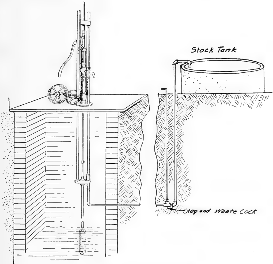
FIG. 356. Piping for stock tank.
