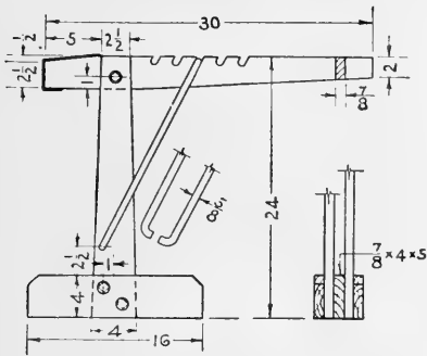
FIG. 133. Wagon jack.
