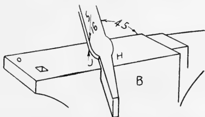
FIG. 241. Shaping the joint of forge tongs.
