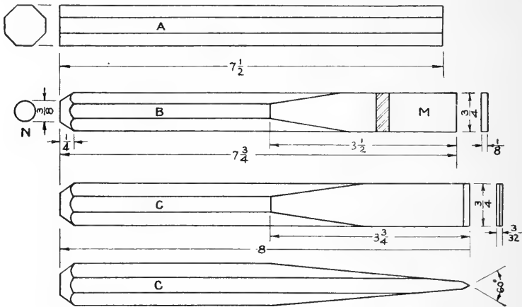
FIG. 223. Cold chisels.
