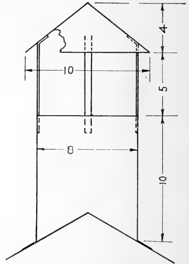
FIG. 301. Roof cap and ventilator.
