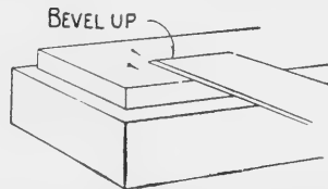
FIG. 56. Whetting the face side of plane-iron.
