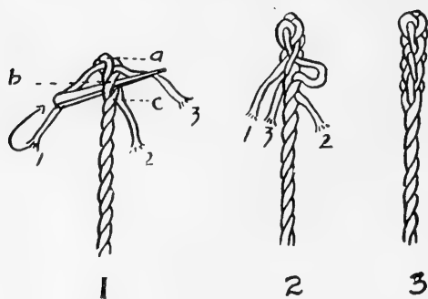
FIG. 369. Crown splice.
