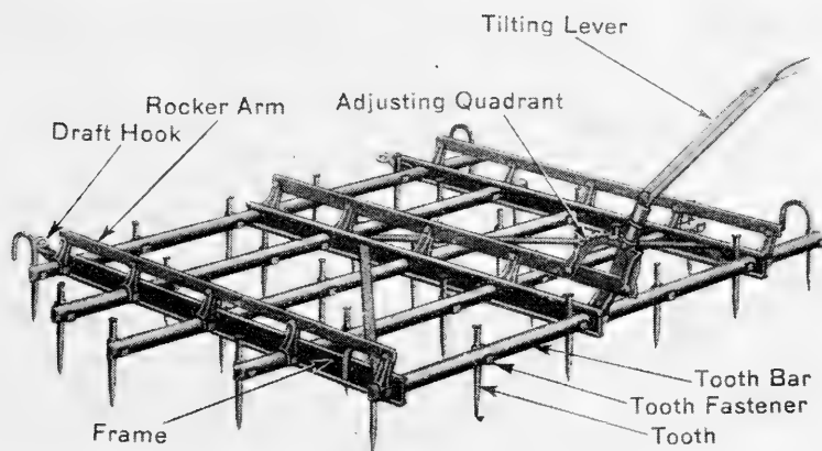
FIG. 317. Peg-toothed harrow.
