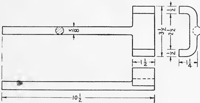
FIG. 207. Wagon wrench.
