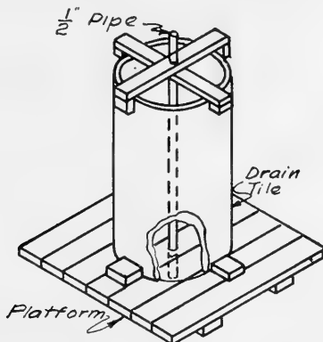
FIG. 157. Details of forms for garden roller.
