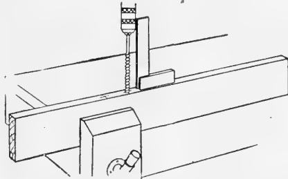
FIG. 34. Testing for squareness when boring.
