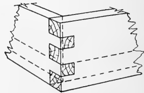
FIG. 102. The bottom fitted inside of side pieces.
