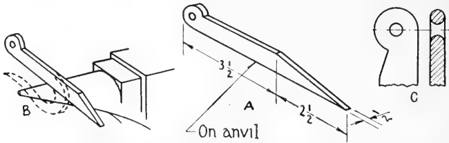
FIG. 202. Further operations in construction of log hook.
