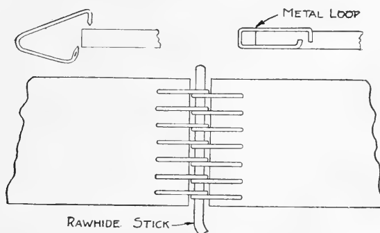
FIG. 337. Hinged belt lacing with wire hooks.
