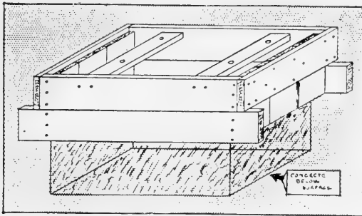
FIG. 159. Machine foundation.
