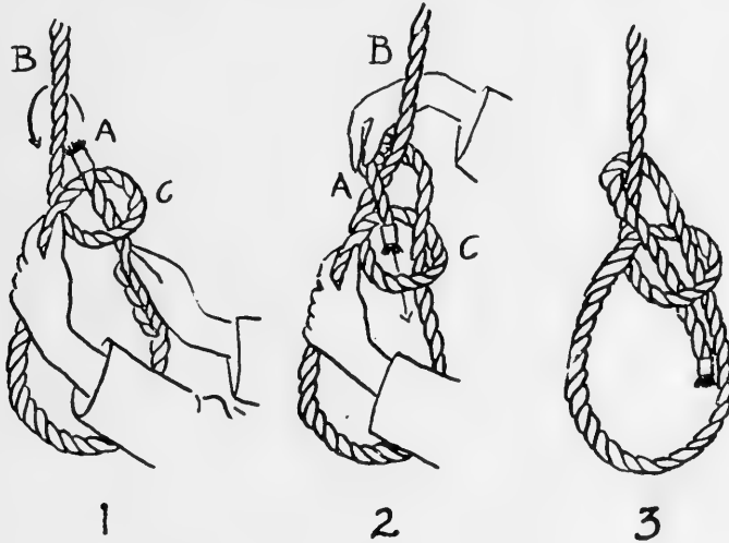
FIG. 380. Bowline knot.
