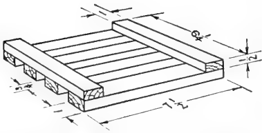
FIG. 13. End of peck crate.
