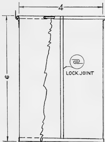
FIG. 279. Small pail.
