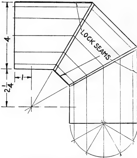
FIG. 300. Three-piece elbow.
