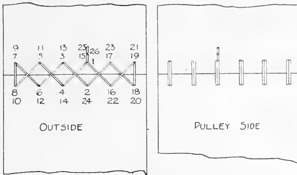
FIG. 335. Wire lacing.
