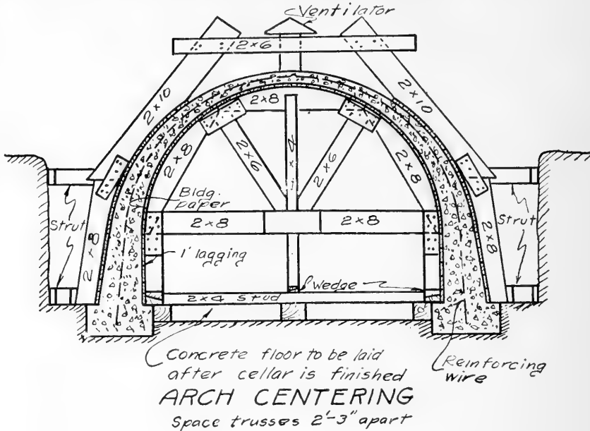
FIG. 168. Fruit storage cellar.
