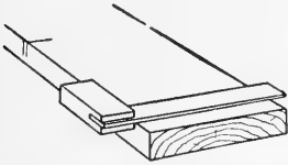
FIG. 19. Position of try-square when squaring face side.
