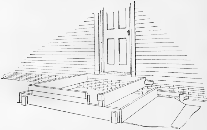
FIG. 149. Form for double step.
