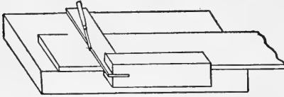
FIG. 327. Squaring a belt.
