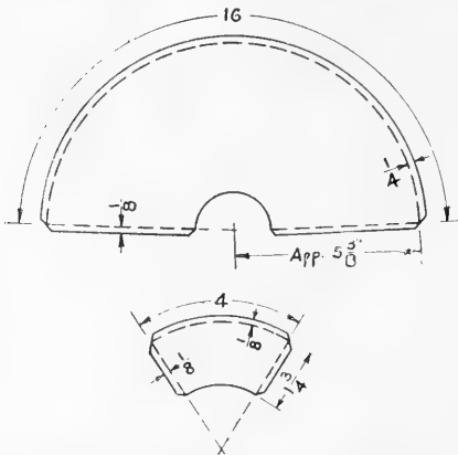
FIG. 290. Metal cut for funnel.
