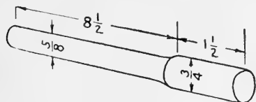
FIG. 214. The handle of the wrench prepared.
