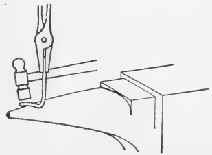
FIG. 185. Forming the point on gate hook.
