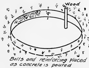
FIG. 160. Earth form for cistern or well top.
