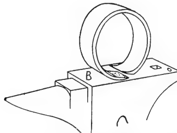
FIG. 231. The ring shaped for welding.
