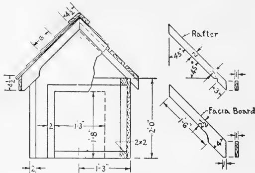
FIG. 120. Dog house.
