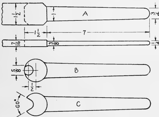
FIG. 197. Steps in making wrench.
