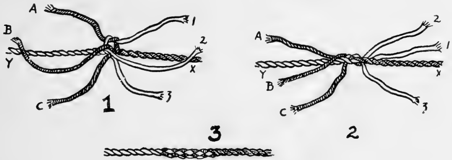
FIG. 397. Shortsplice.
