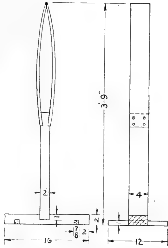
FIG. 86. Harness clamp.
