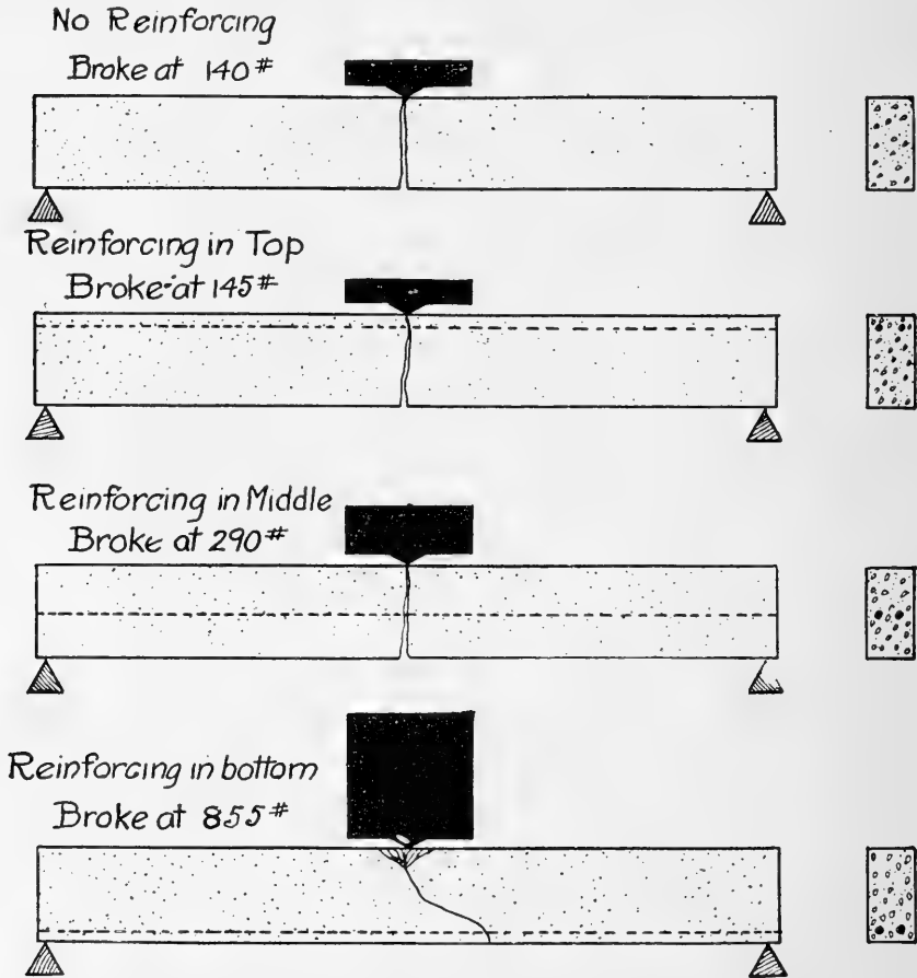
FIG. 144. Results of different placing of reinforcing.
