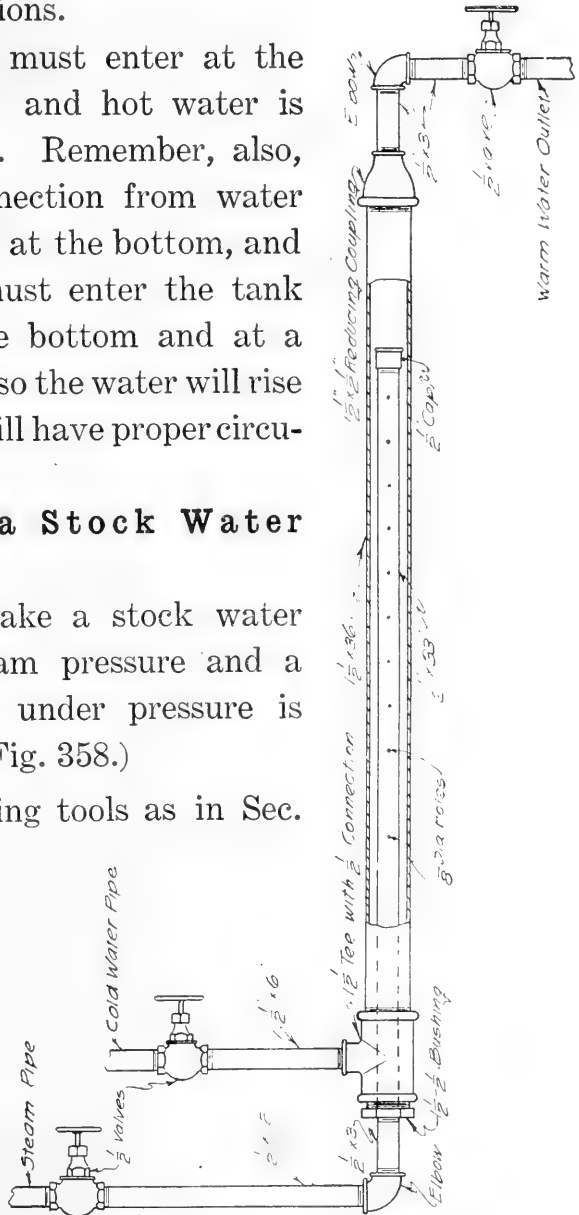
FIG. 358. Stock water heater.
