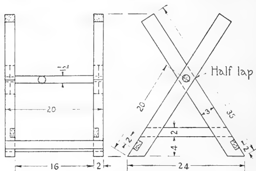
FIG. 127. Saw buck.
