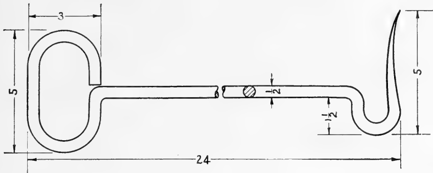
FIG. 180. Stove poker.
