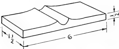
FIG. 213. Preparing wagon wrench for welding.
