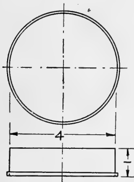
FIG. 292. Cylindrical receptacle.
