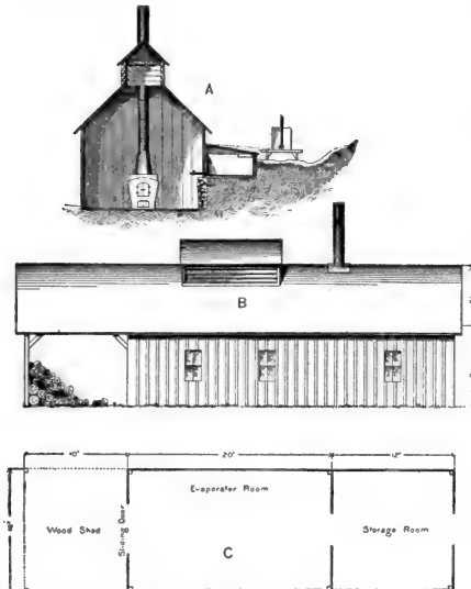
FIG. 53. — Plan of model sugarhouse: A , sectional view showing evaporator, storage tank, and gathering tank (on sled). B , elevation. C , ground plan.
