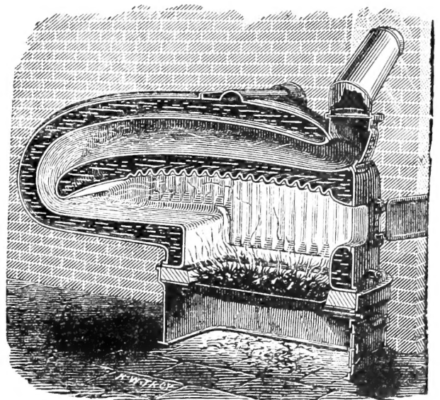
Our Well-known Corrugated Fire-Box Boiler.
