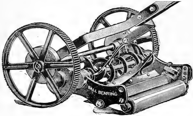
Victory Ball Bearing.
