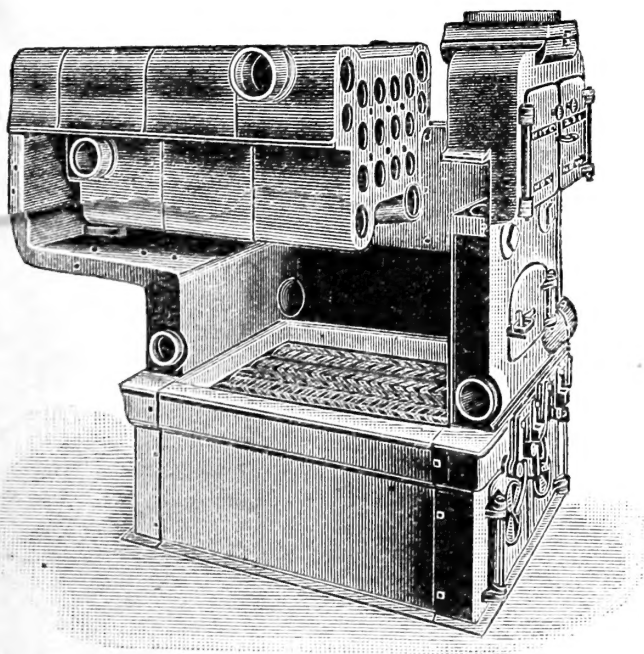
Our New Sectional Tubular Boiler.
