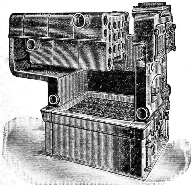
Our New Sectional Tubular Boiler.
