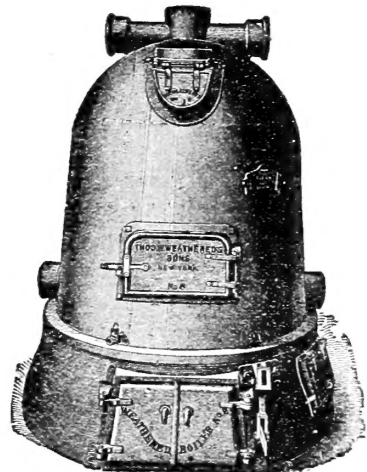
Conical Boilers in 5 Sizes. Capacity 250 to 1500 feet, 4 inch pipe.
