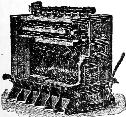
Sectional Boilers of Various Sizes. Capacity 1100 to 7,000 feet, 4 inch pipe.
